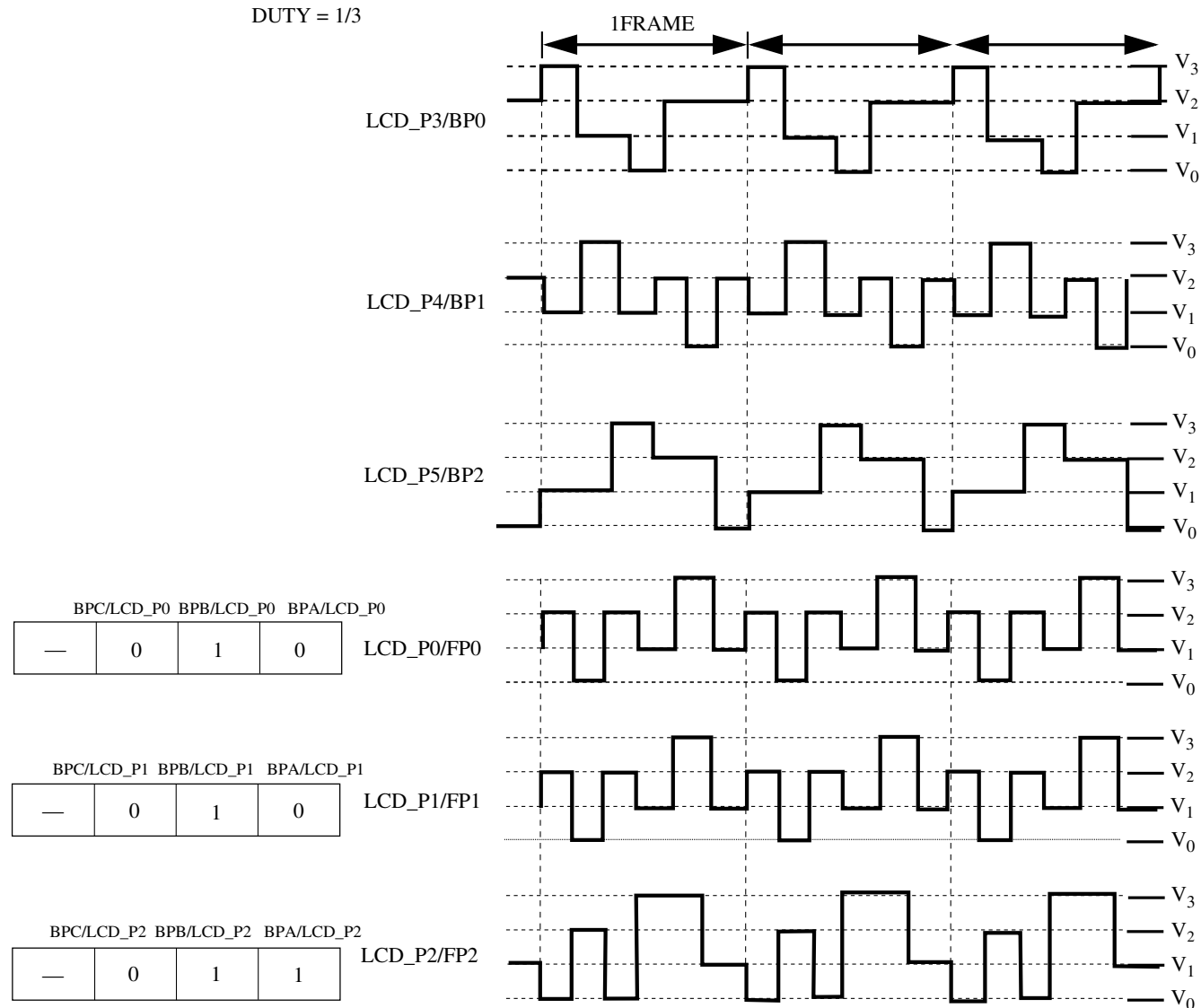
Figure 49-40. LCD waveforms
