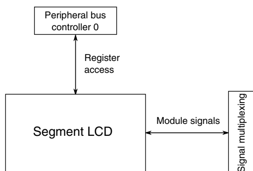
Figure 3-54. SLCD configuration
