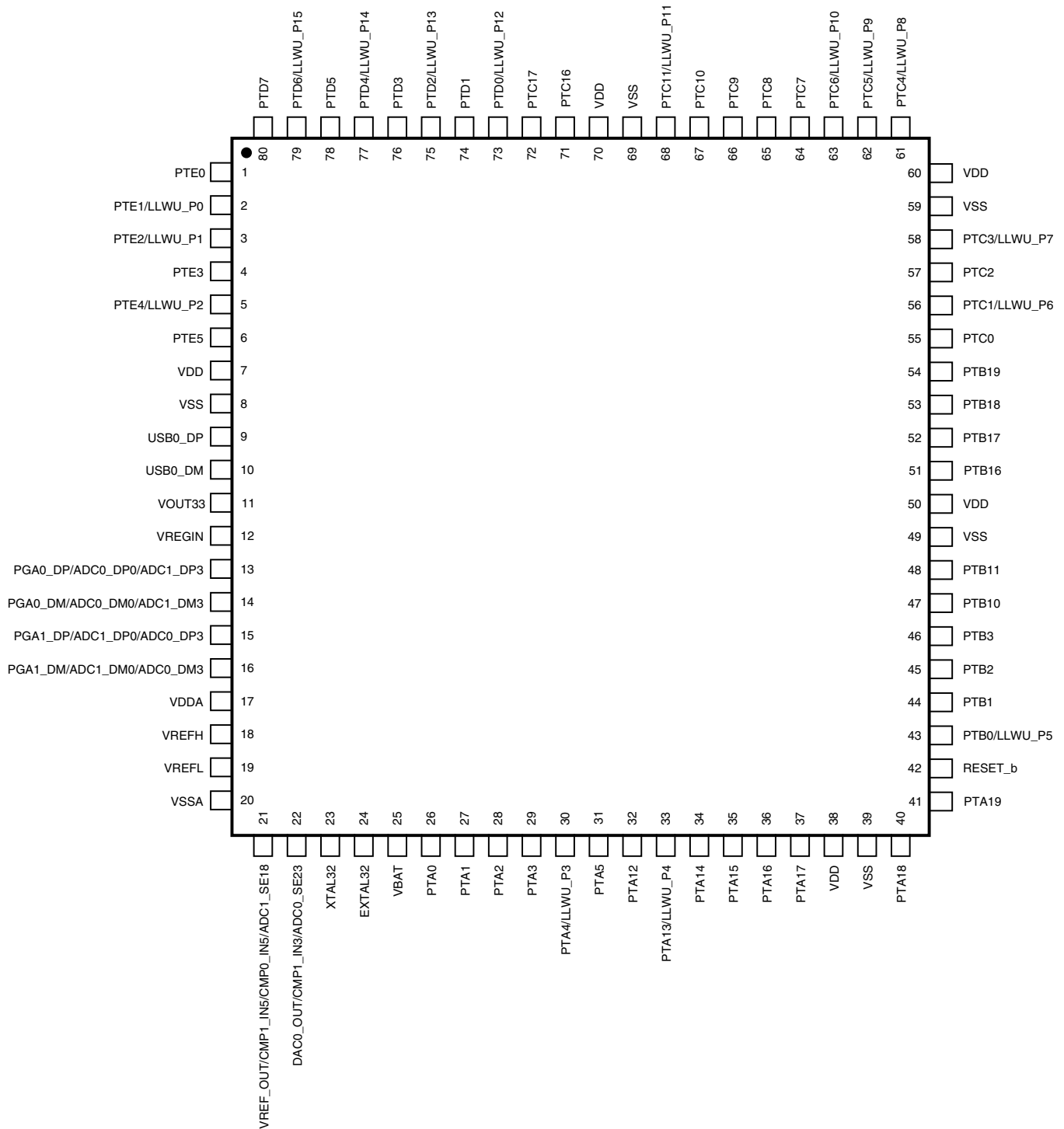
Figure 10-2. K20 80 LQFP Pinout Diagram
