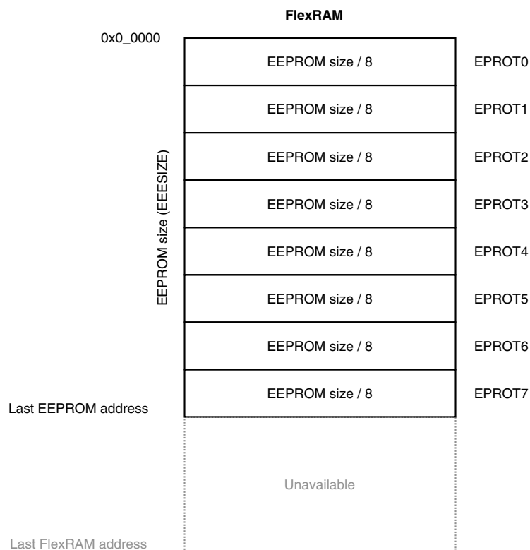
Figure 28-30. EEPROM protection
