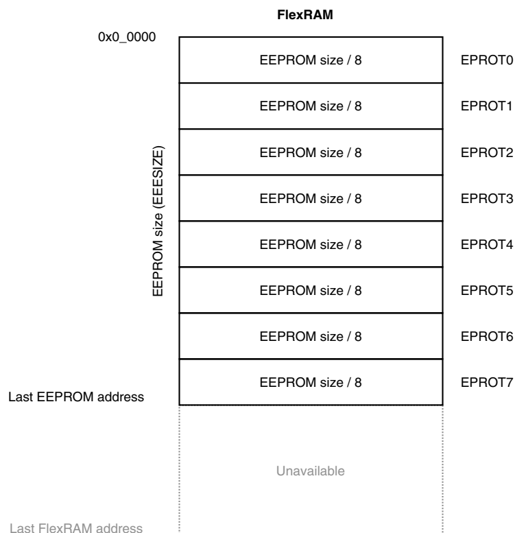
Figure 28-29. EEPROM protection
