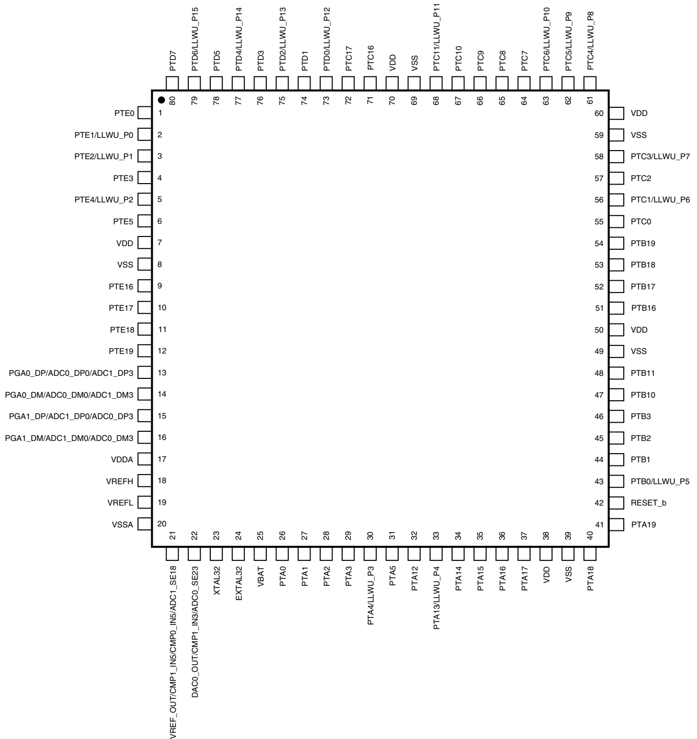
Figure 10-2. K10 80 LQFP Pinout Diagram
