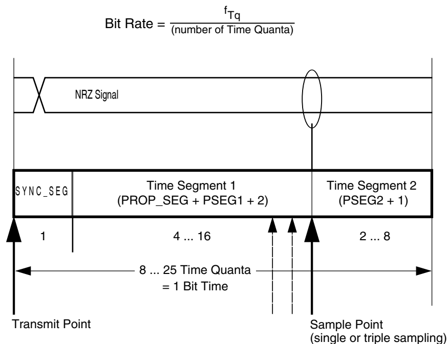
Figure 42-105. Segments within the Bit Time
