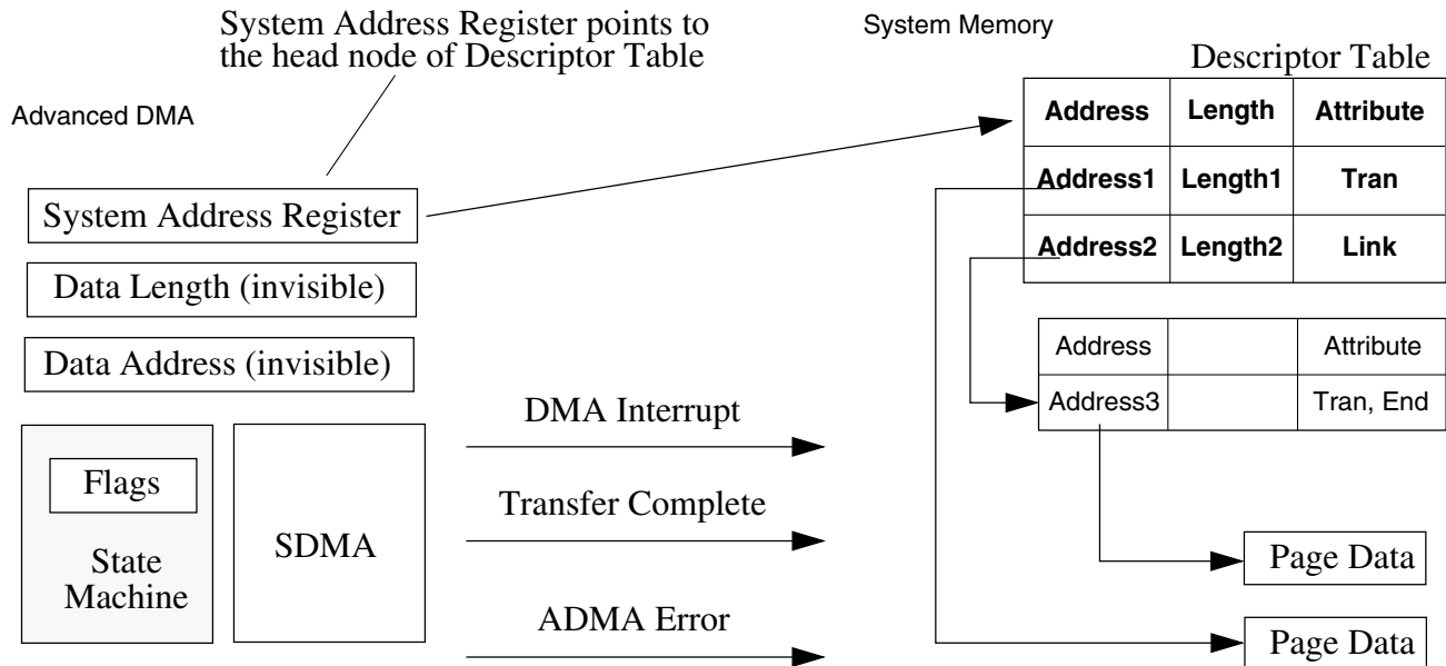
Figure 46-33. Concept and access method of ADMA2 descriptor table
