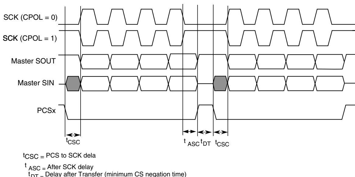
Figure 43-74. Example of Non-Continuous Format (CPHA=1, CONT=0)
