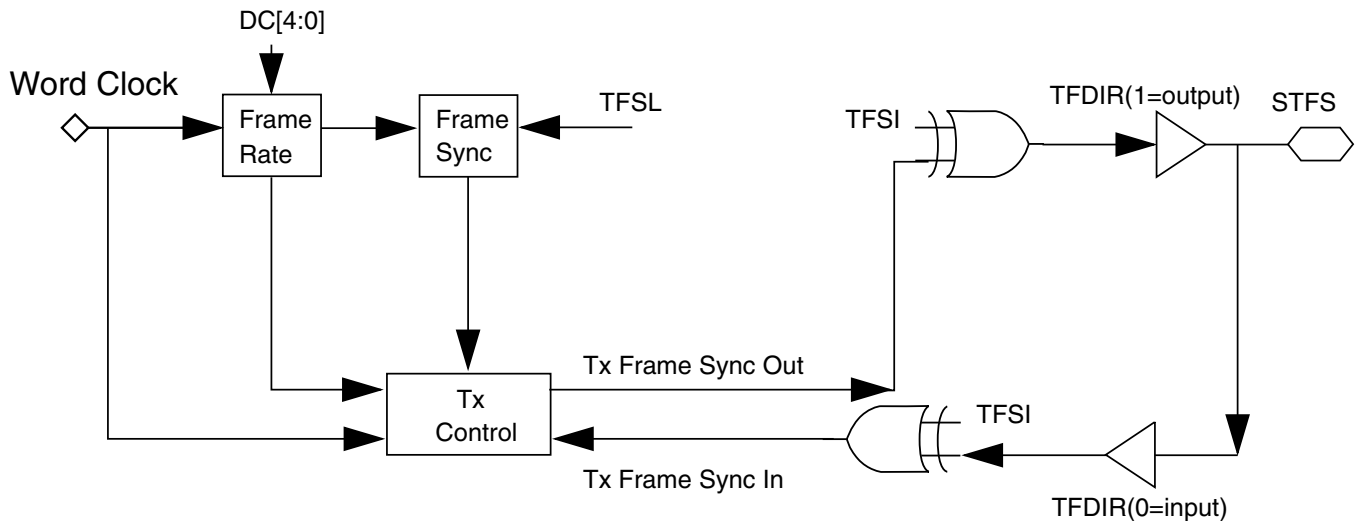
Figure 47-57. I²S transmit frame sync generator block diagram
