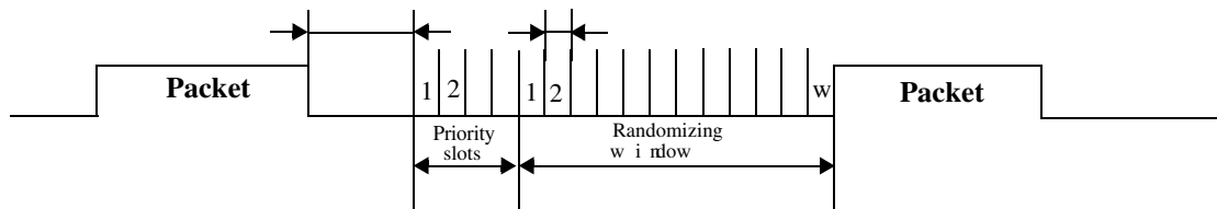
Figure 45-51. CEA709.1-B packet cycle
