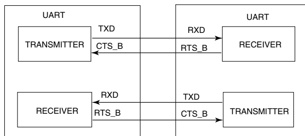
Figure 45-74. Ready-to-receive
