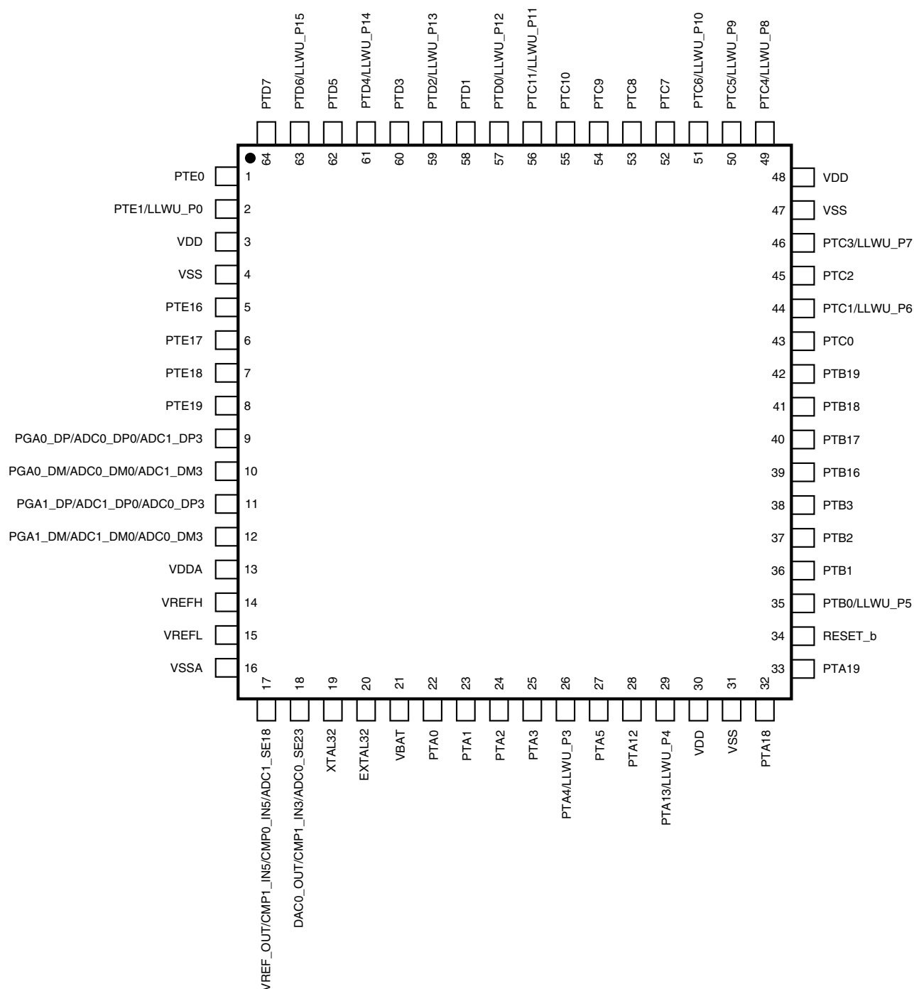
Figure 10-2. K10 64 LQFP/QFN Pinout Diagram
