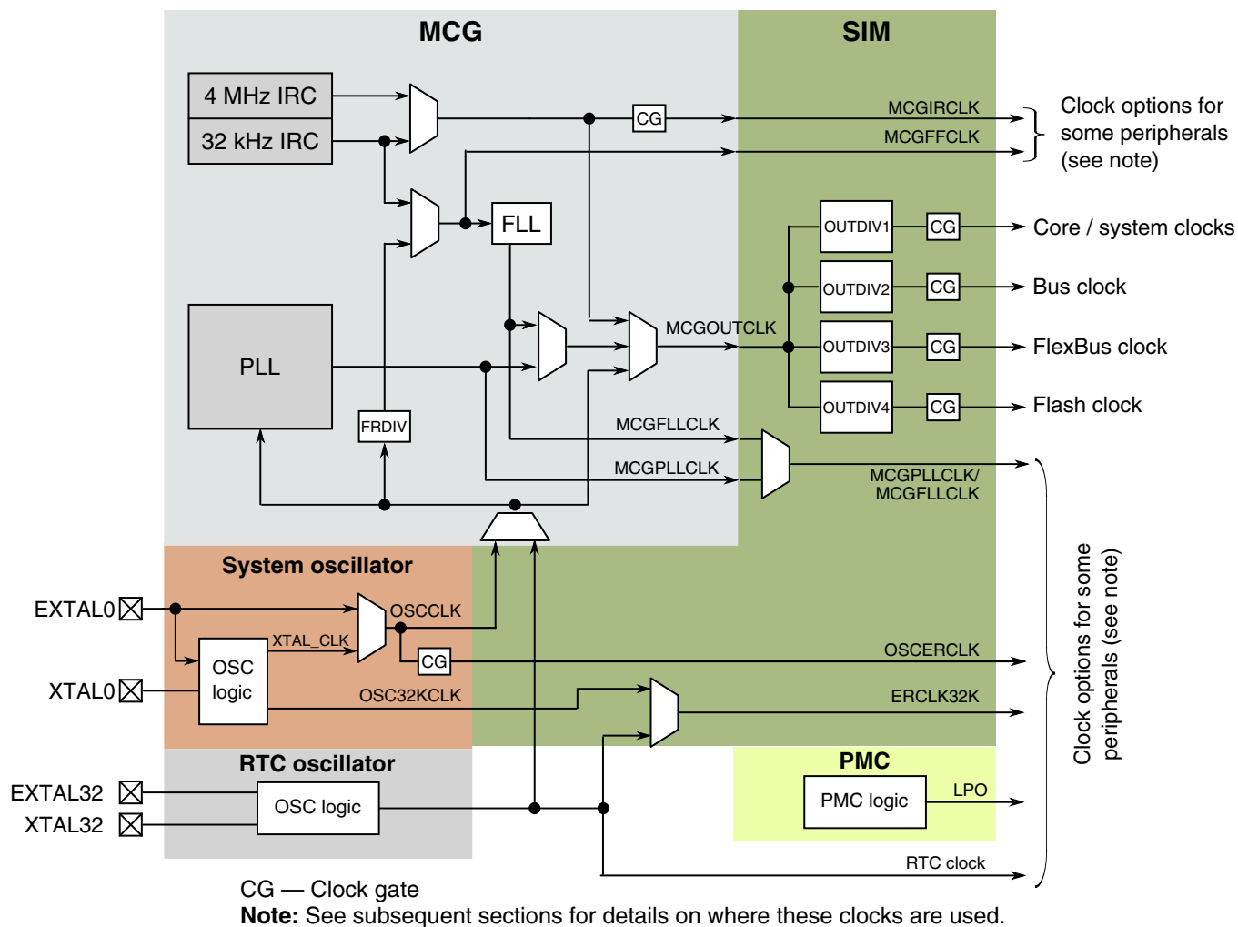
Figure 5-1. Clocking diagram
