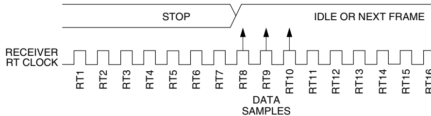
Figure 45-59. Fast data
