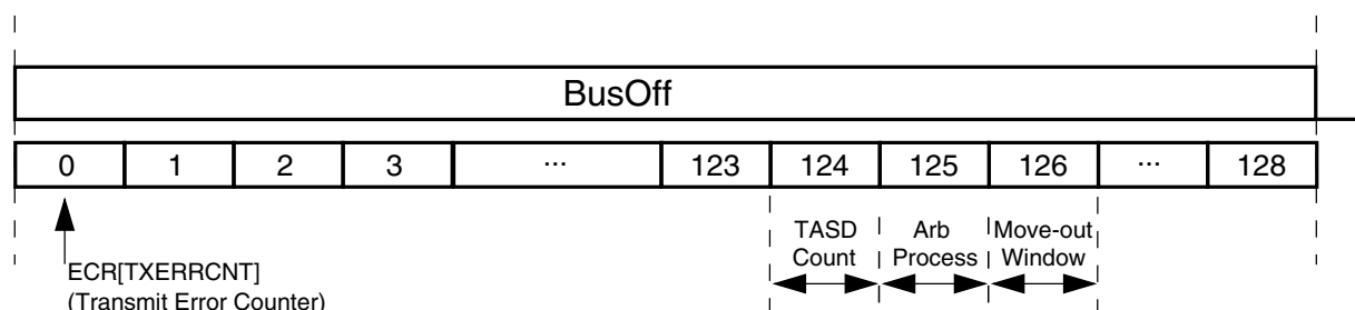
Figure 42-70. Arbitration at the end of bus off and move-out time windows
