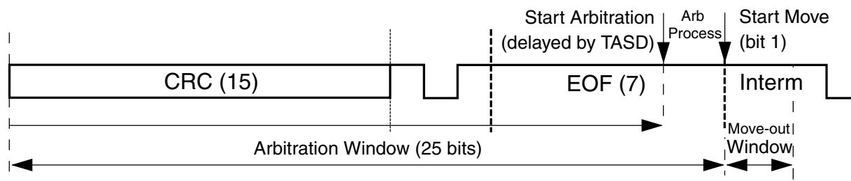
Figure 42-69. Arbitration and move-out time windows
