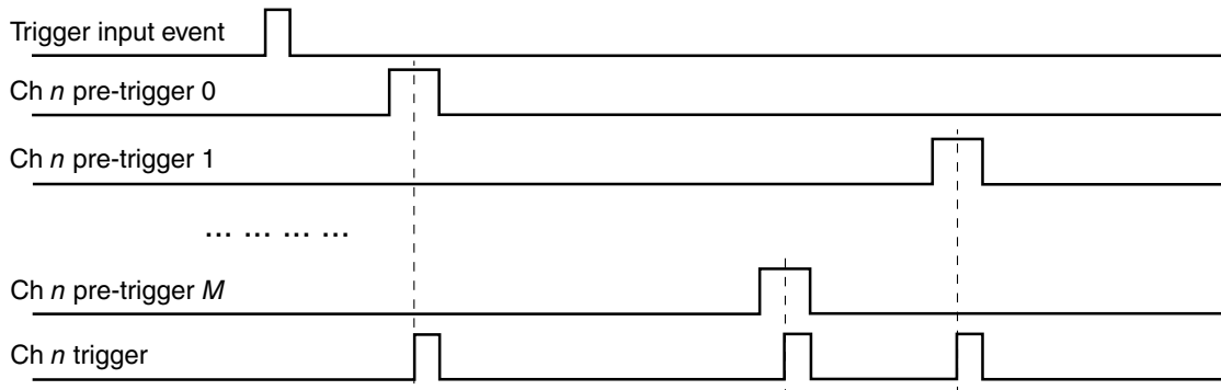
Figure 36-52. Pre-trigger and trigger outputs
