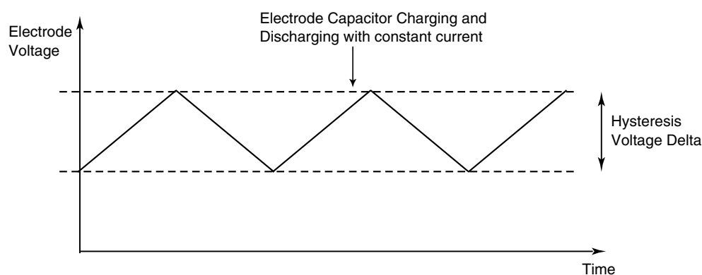
Figure 48-34. TSI electrode oscillator chart
