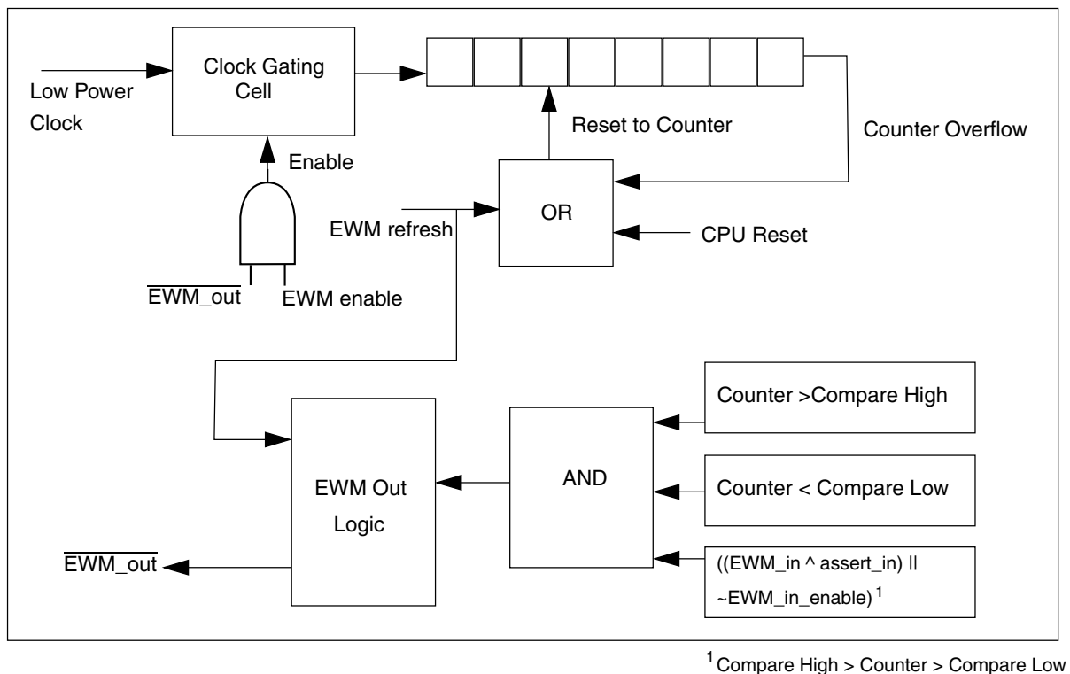
Figure 22-1. EWM Block Diagram
