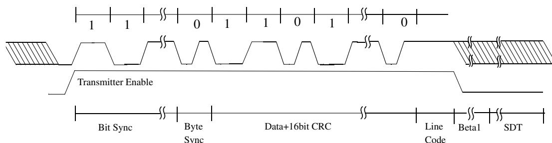
Figure 46-337. Frame format with differential manchester encoding
