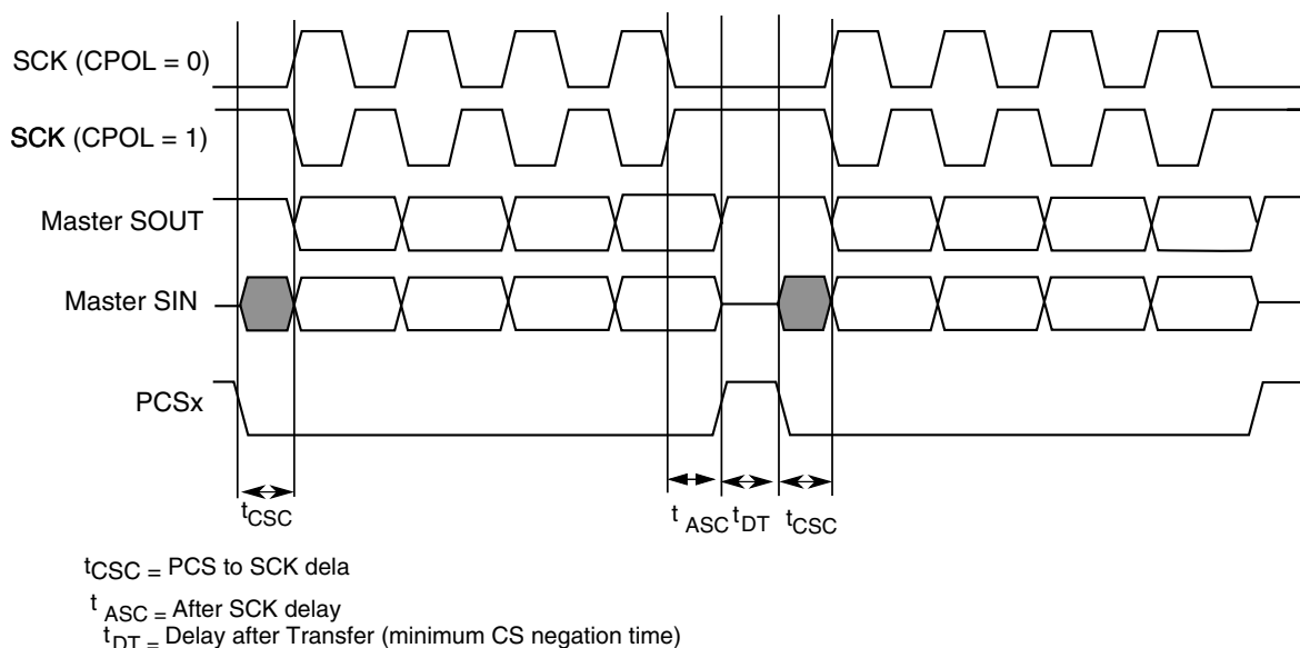
Figure 44-95. Example of non-continuous format (CPHA=1, CONT=0)
