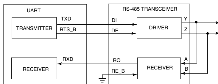
Figure 46-363. Transceiver driver enable using RTS
