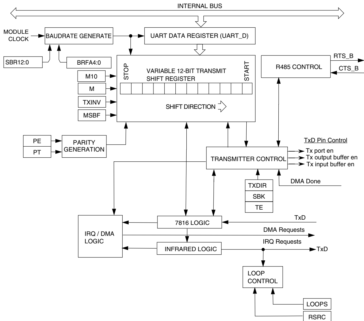
Figure 46-342. Transmitter Block Diagram
