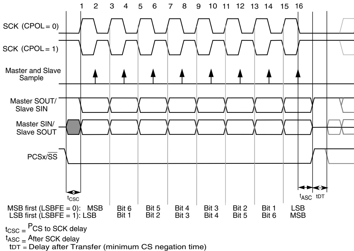
Figure 44-94. Module transfer timing diagram (MTFE=0, CPHA=1, FMSZ=8)
