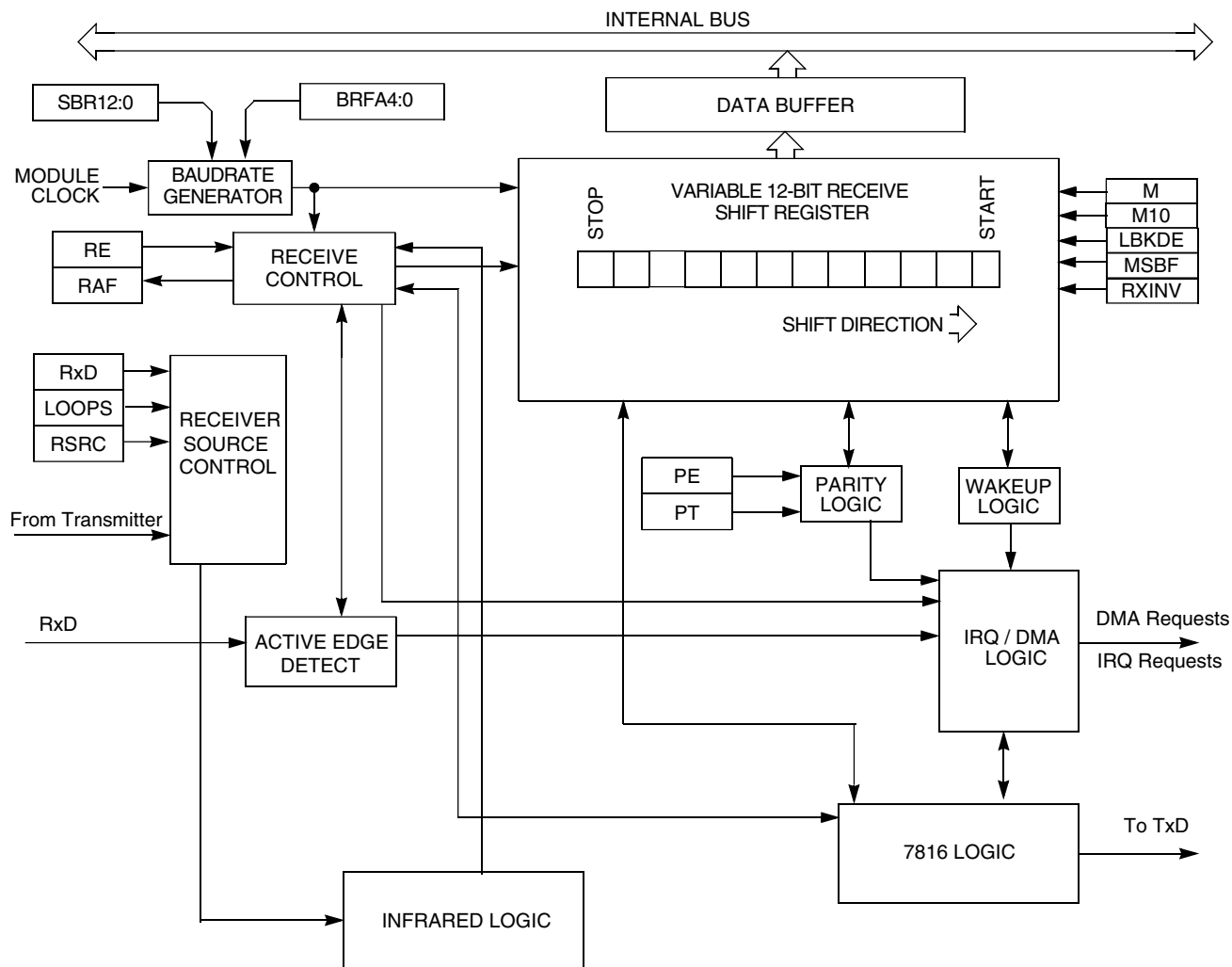
Figure 46-344. UART receiver block diagram
