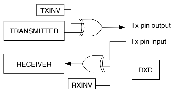
Figure 46-358. Single-wire operation (C1[LOOPS] = 1, C1[RSRC] = 1)
