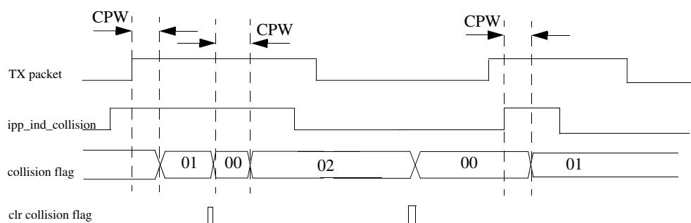
Figure 46-341. Collision pulse detection
