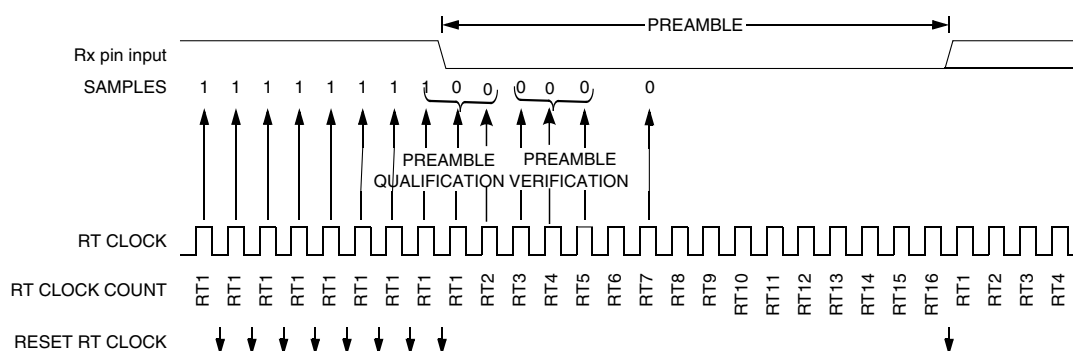
Figure 46-340. Receiver data sampling
