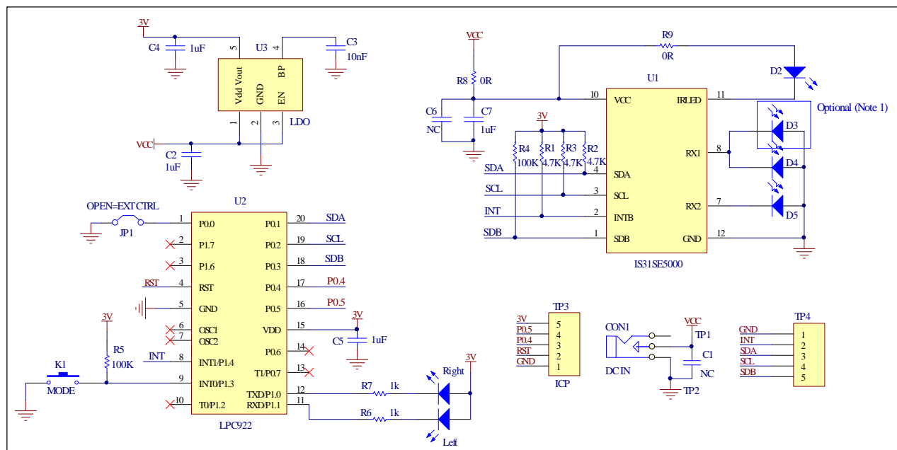
Figure 2: IS31SE5000 Application Schematic
