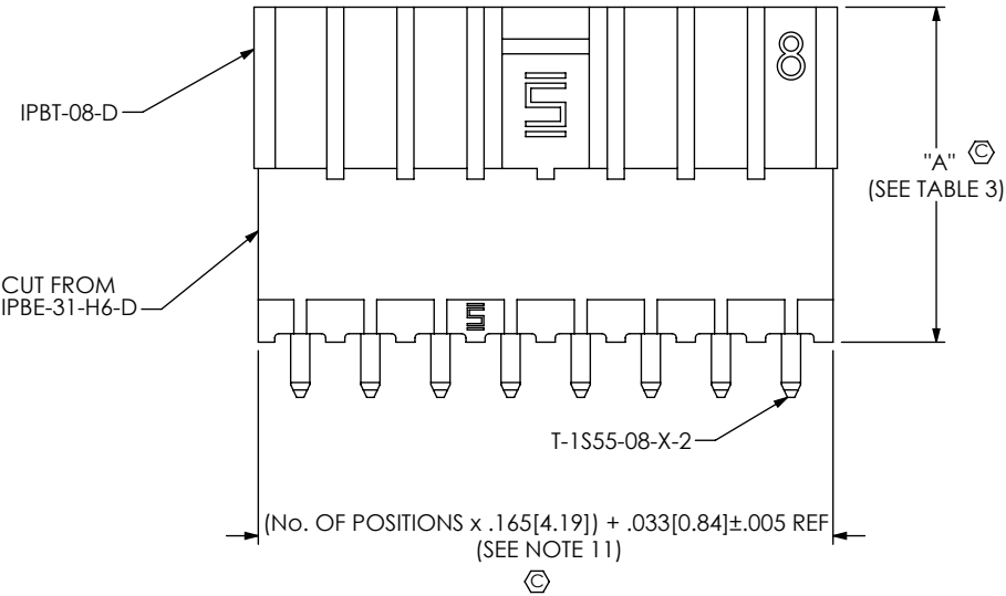
FIG 6 (IPBT-108-H6-XX-D SHOWN) (DIFFERENT AS SHOWN, OTHERWISE SAME AS FIG. 1)
