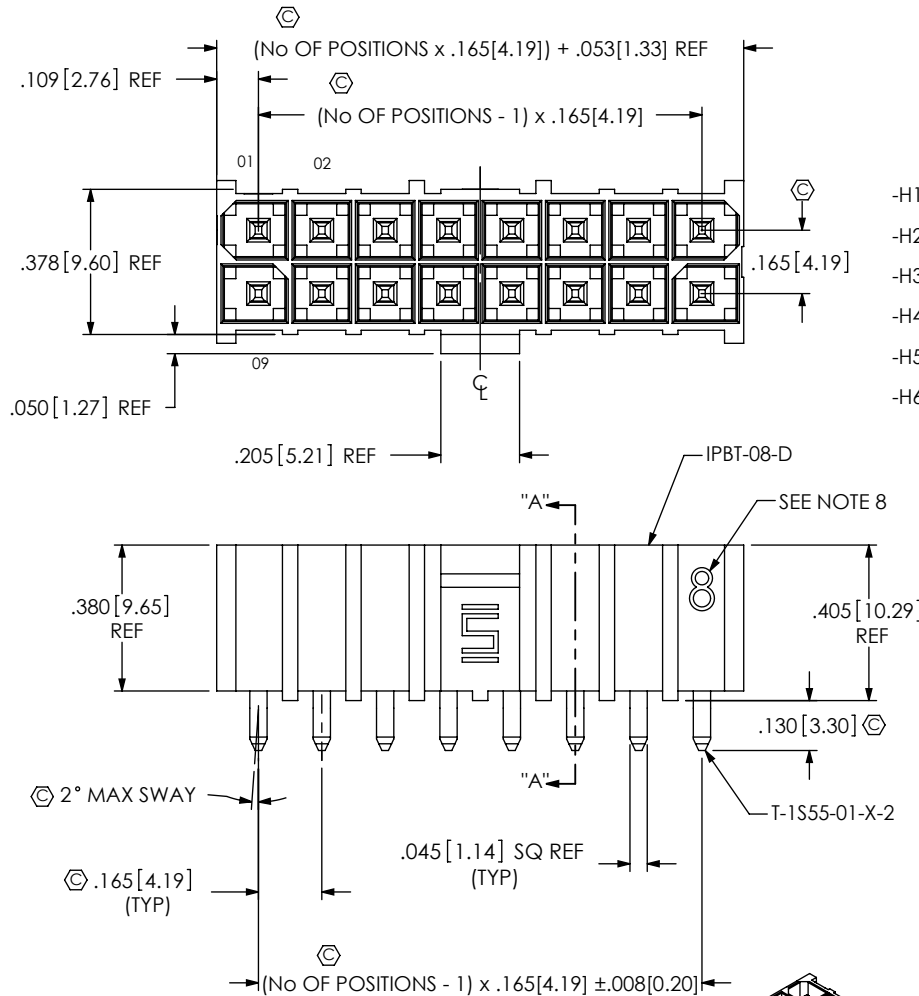
FIG 1 (IPBT-108-HT-XX-D SHOWN)
