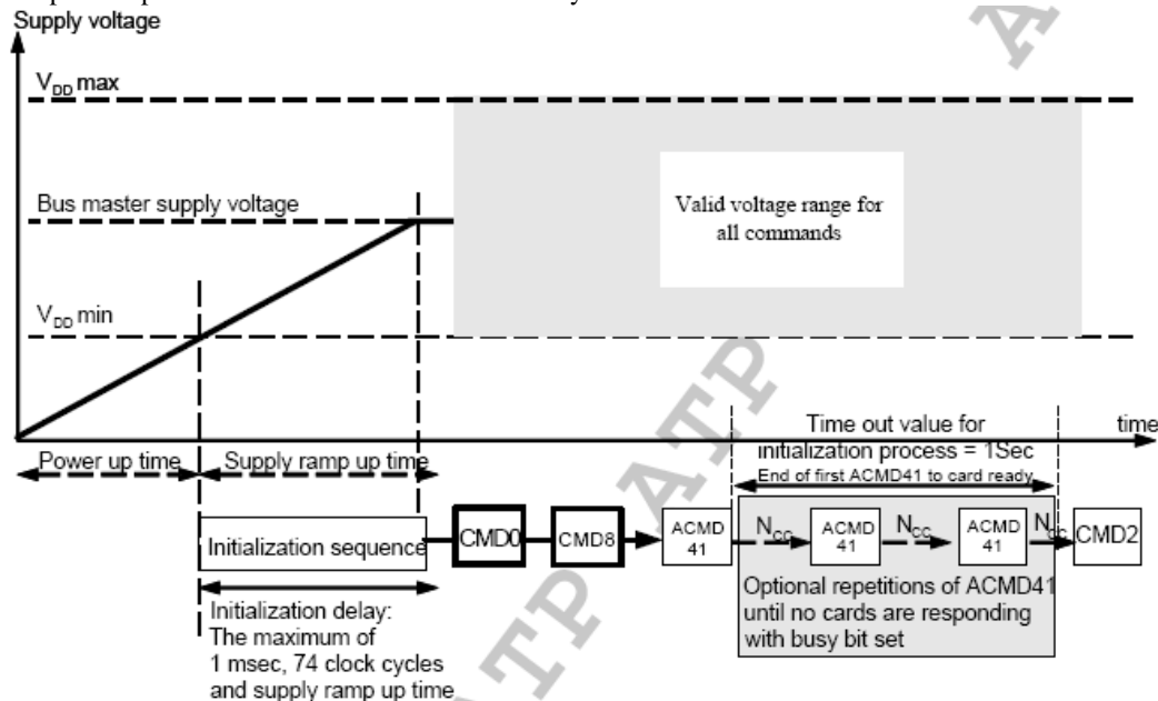
Figure 4-4: Power-up diagram
