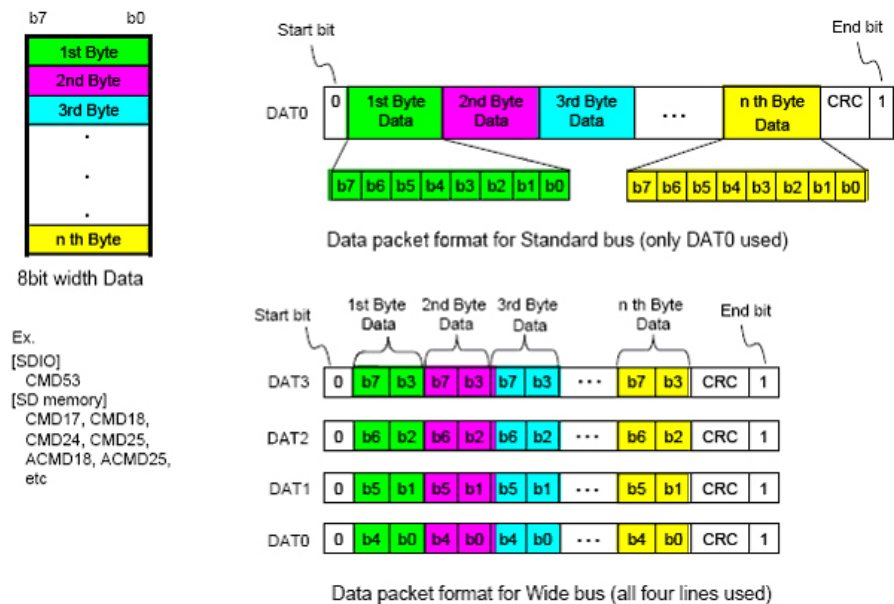
Figure 6-6: Data packet format - Usual data
