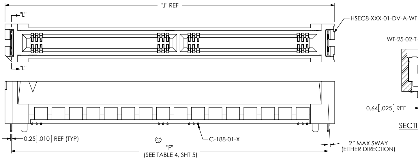
FIG 8 ** -WT: WELD TAB OPTION HSEC8-160-01-XX-DV-A-WT SHOWN AVAILABLE IN ALL POSITIONS (-A OPTION REQUIRED) (DIFFERENT AS SHOWN, OTHERWISE SAME AS FIG 2) (SOME FEATURES NOT SHOWN FOR CLARITY) ** = AVAILABLE ONLY WITH -01 CARD THICKNESS
