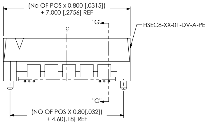
FIG 7 ** -PE: PASS THROUGH OPTION HSEC8-120-01-XX-DV-A-PE SHOWN AVAILABLE IN -10, *-13 & -20 POSITIONS ONLY (DIFFERENT AS SHOWN, OTHERWISE SAME AS FIG 1) (SOME FEATURES NOT SHOWN FOR CLARITY) ** = AVAILABLE ONLY WITH -01 CARD THICKNESS *-13 IS A ONE BANK PART
