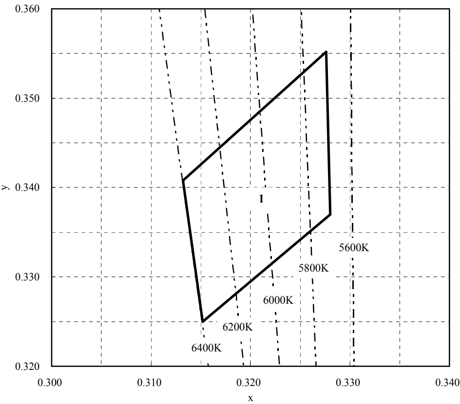
Chromaticity Diagram
