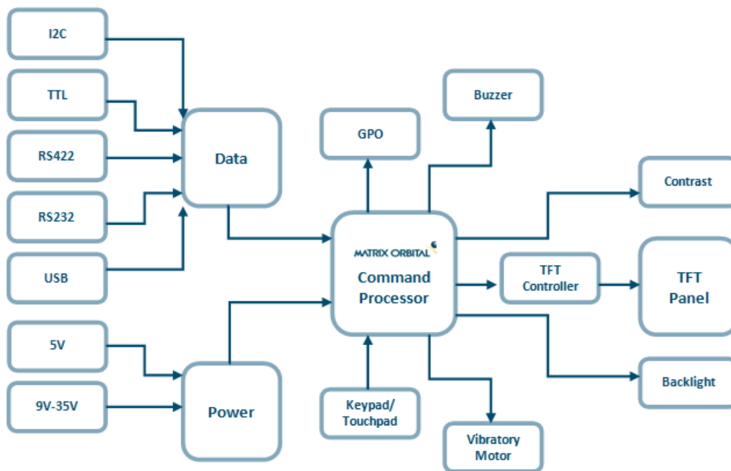
Figure 2: Functional Diagram
