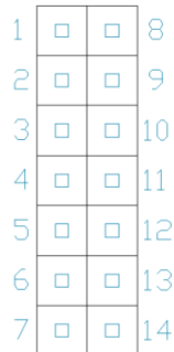
Figure 15: GPO Header
