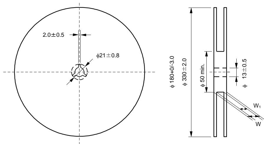
Fig.3 Taping Diagram
