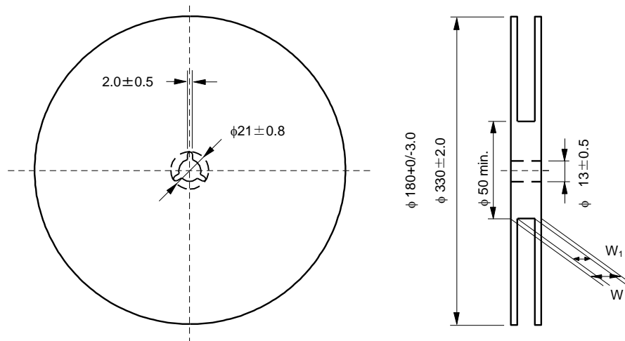
Fig.3 Taping Diagram
