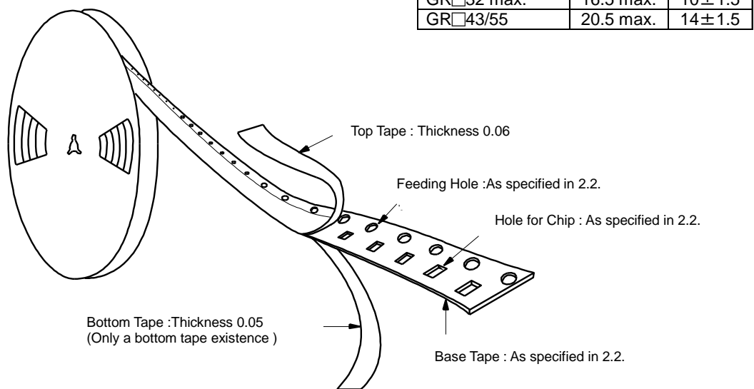
Fig.3 Taping Diagram
