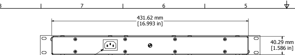
ASSEMBLY - VIEW FROM BACK
