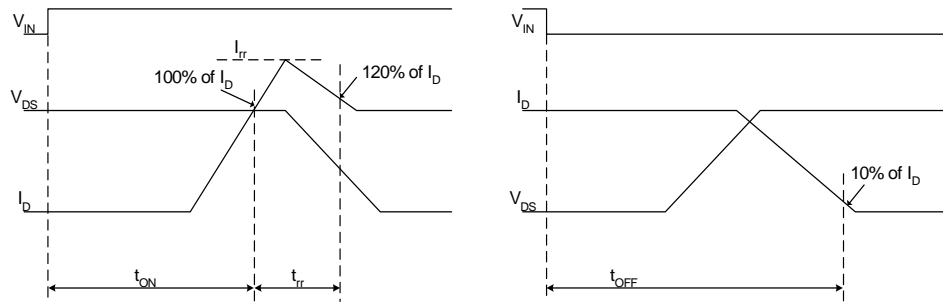
Figure 6. Switching Time Definitions
