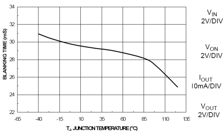
Figure 17. t_{\text{BLANK}} vs. Temperature
