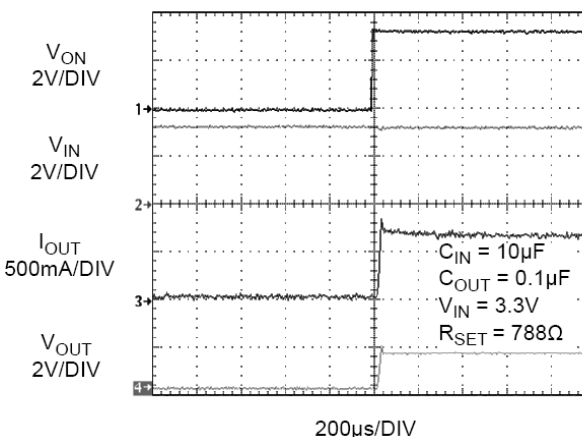
Figure 22. Current Limit Response Time (Output is Loaded by 2.2 \Omega , C_{\text{OUT}} = 0.1\mu\text{F} )
