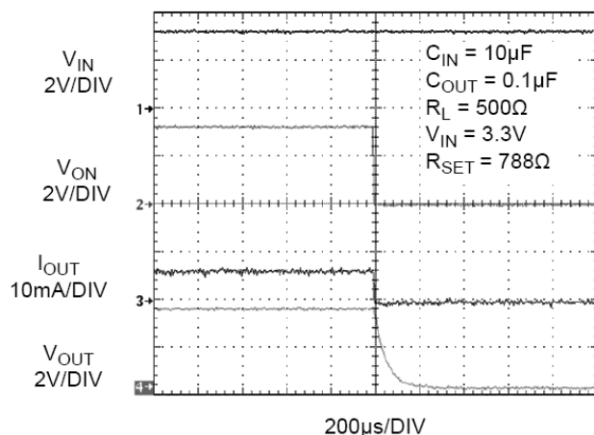
Figure 19. t_{\text{OFF}} Response
