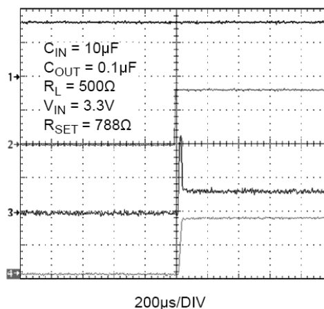
Figure 18. t_{\text{ON}} Response
