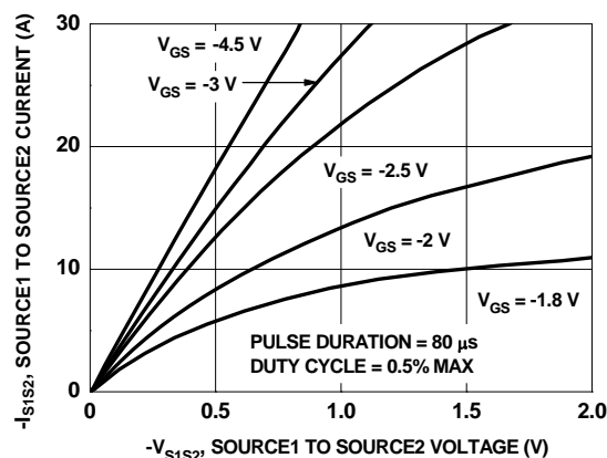
Figure 2. On-Region Characteristics
