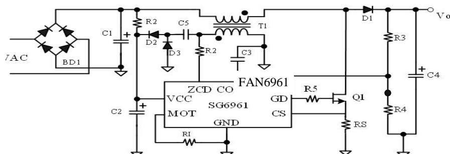
Figure 1. Typical Application
