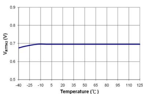
Figure 22. Over-Temperature Protection Threshold Voltage (V RTTH2 ) vs. Temperature
