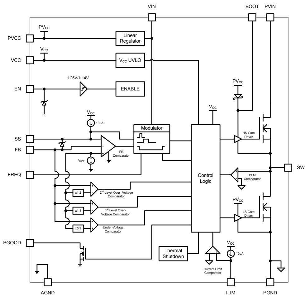
Figure 3. Block Diagram
