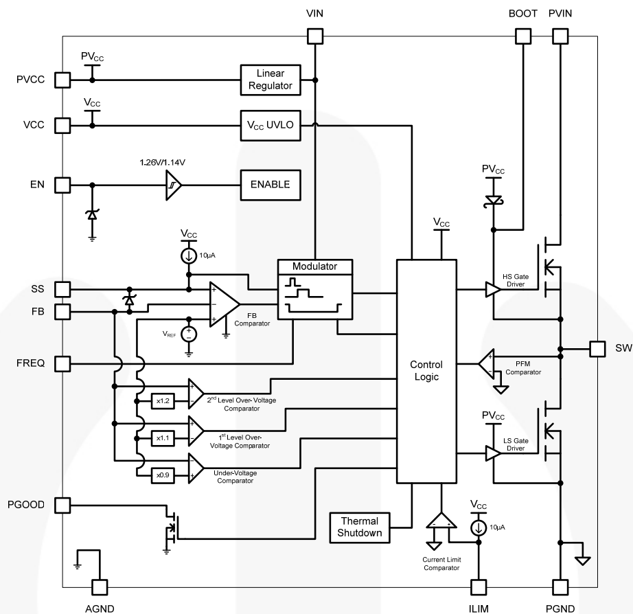
Figure 3. Block Diagram
