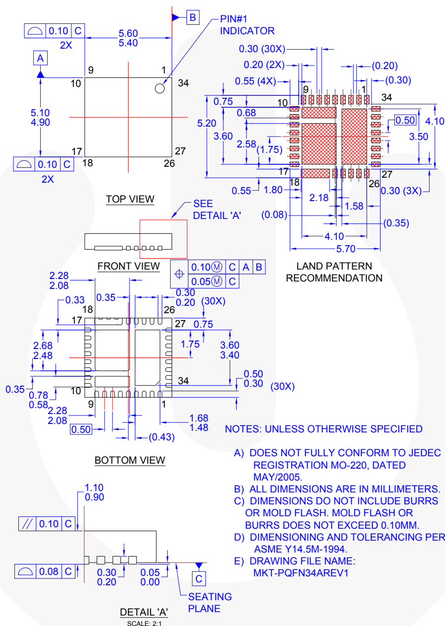
Figure 30. 34-Lead, PQFN, 5.5 mm x 5.0 mm Package
