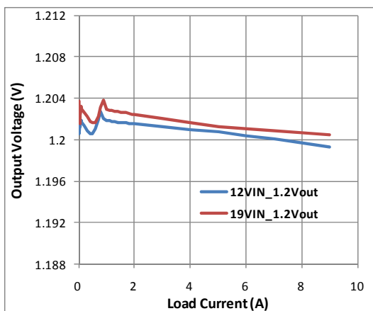
Figure 12. Load Regulation
