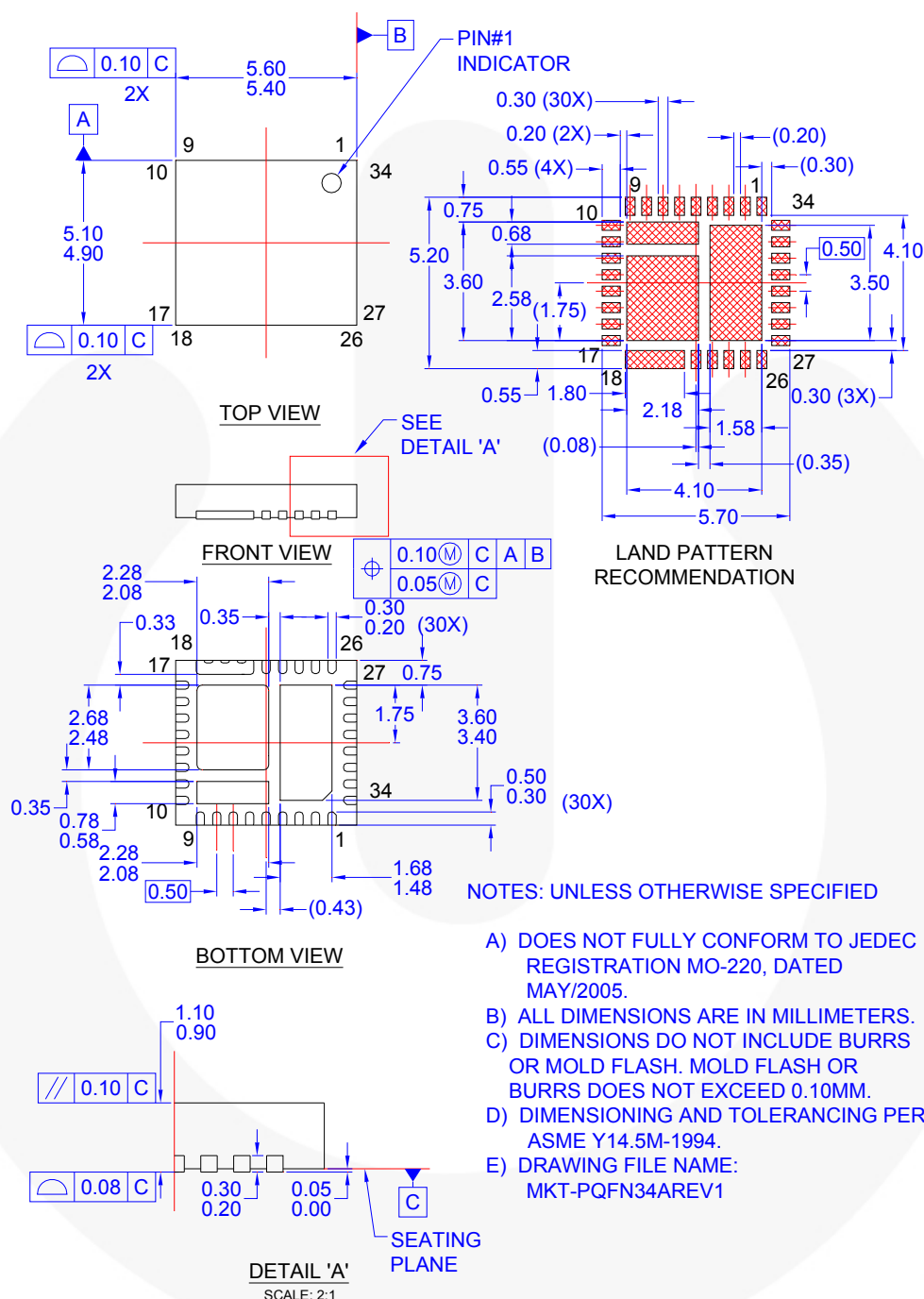
Figure 30.34-Lead, PQFN, 5.5 mm x 5.0 mm Package
