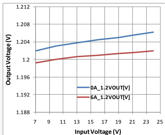
Figure 13. Line Regulation
