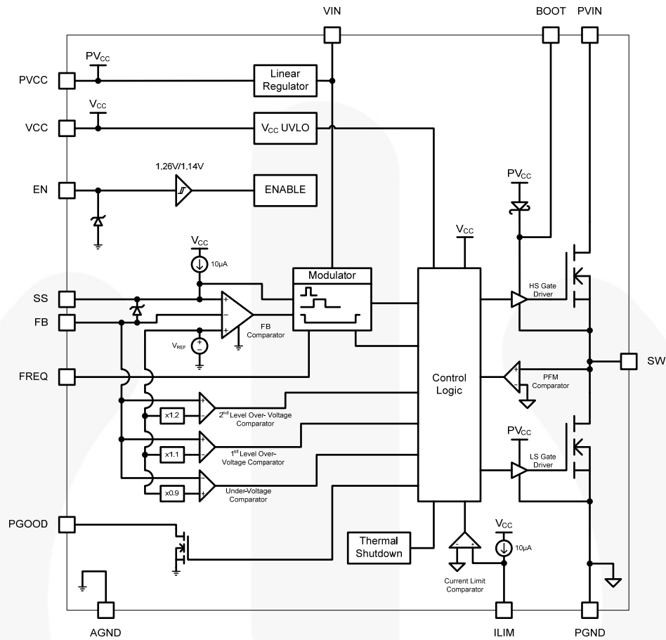
Figure 3. Block Diagram
