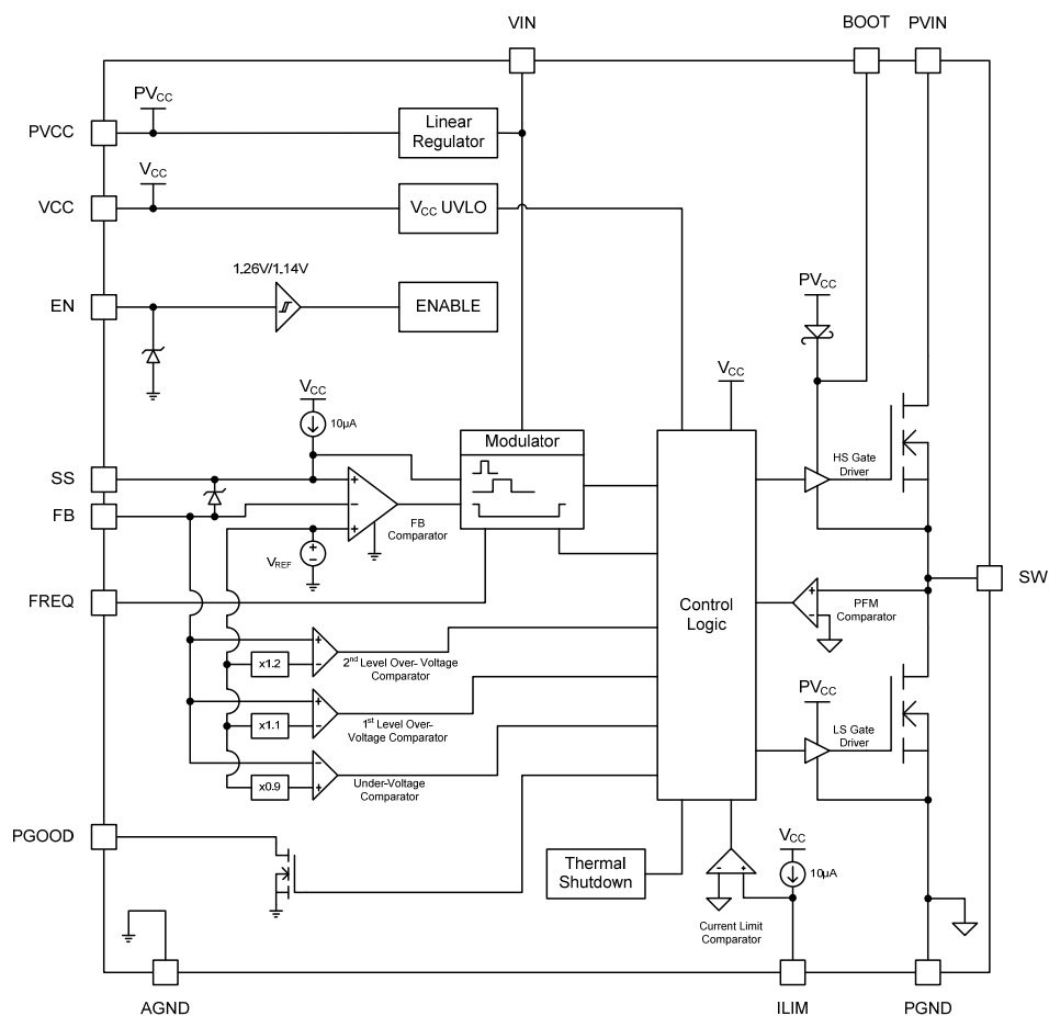
Figure 3. Block Diagram
