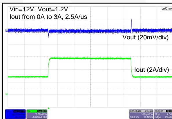
Figure 27. Load Transient from 50% to 100% Load Current
