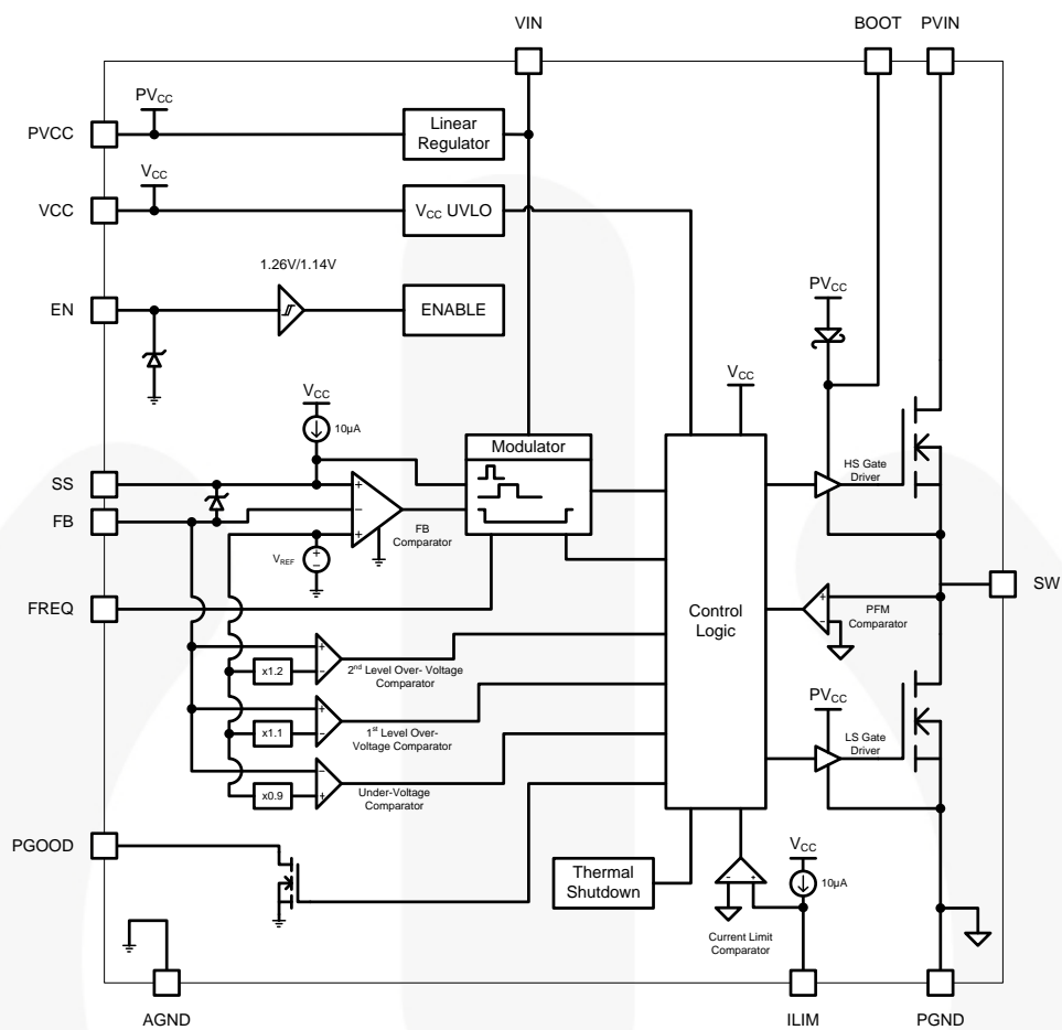
Figure 3. Block Diagram
