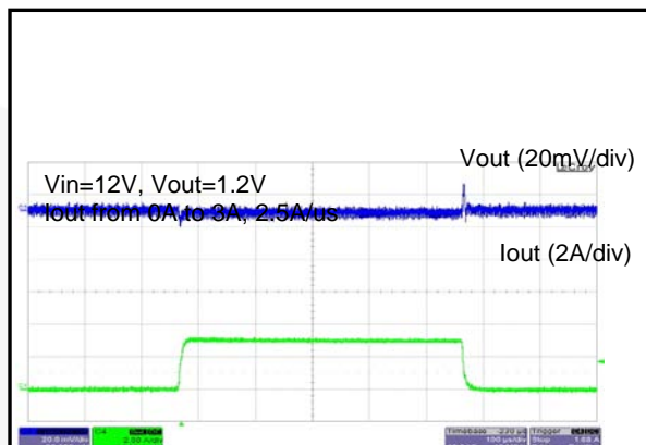
Figure 25. FAN23SV06P Load Transient from 0% to 50% Load Current
