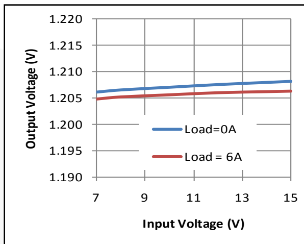
Figure 13. Line Regulation
