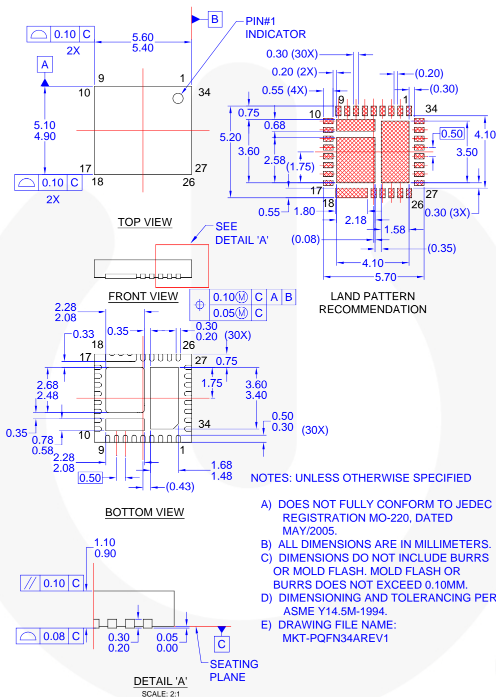
Figure 34.34-Lead, PQFN, 5.5 mm x 5.0 mm Package
