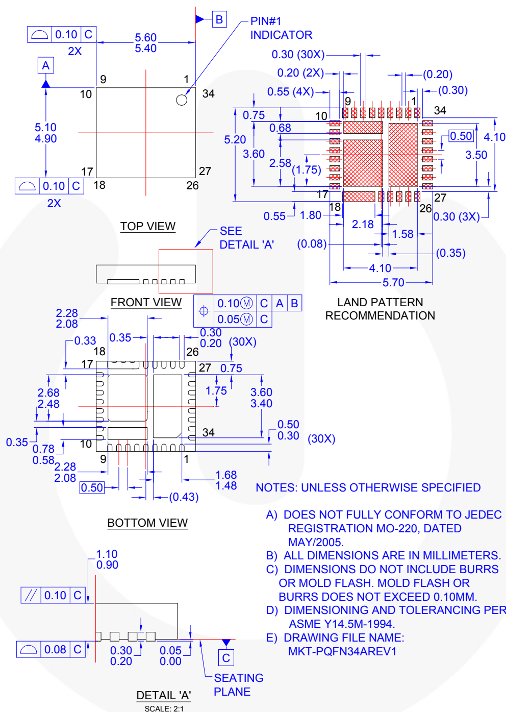
Figure 34. 34-Lead, PQFN, 5.5 mm x 5.0 mm
