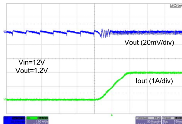
Figure 23. FAN2306 Transition from DCM to CCM
