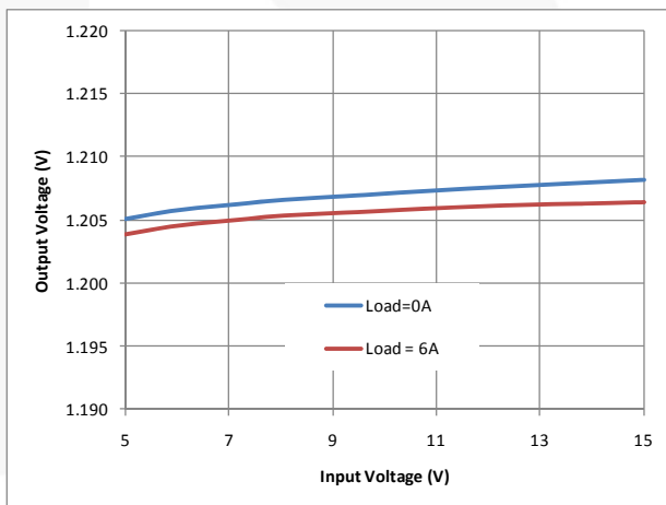
Figure 14. Line Regulation
