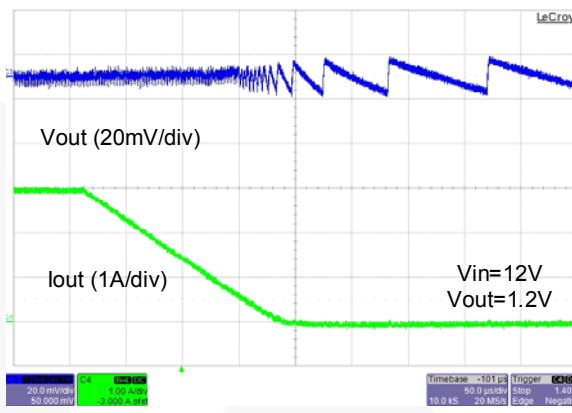
Figure 18. FAN2306M Transition from CCM to DCM
