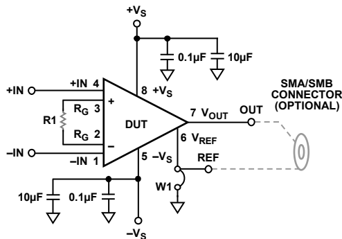
Figure 3. EVAL-INAMP-82RZ Schematic
