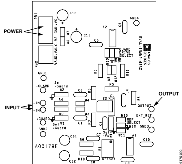
Figure 2. Component Location for the EVAL-INAMP-62
