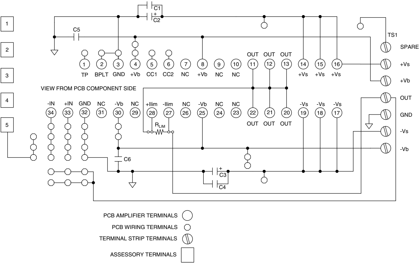
FIGURE 1: SCHEMATIC DIAGRAM
