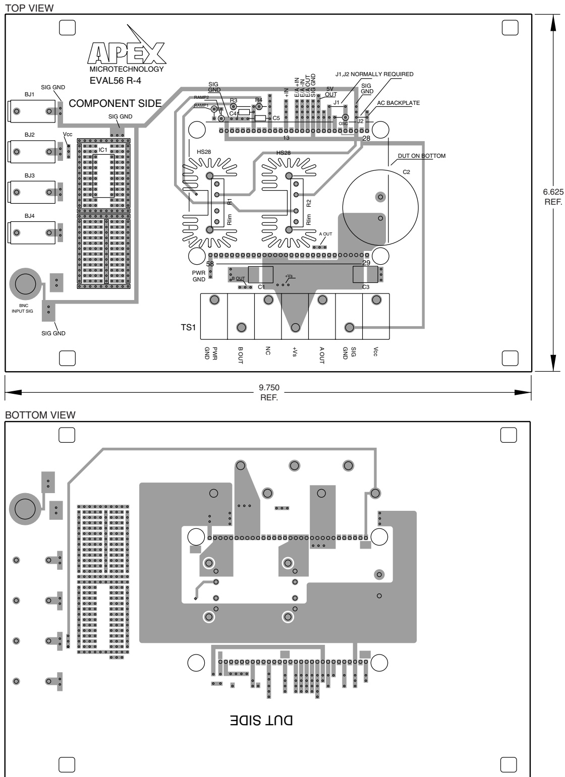
FIGURE 2: PCB
