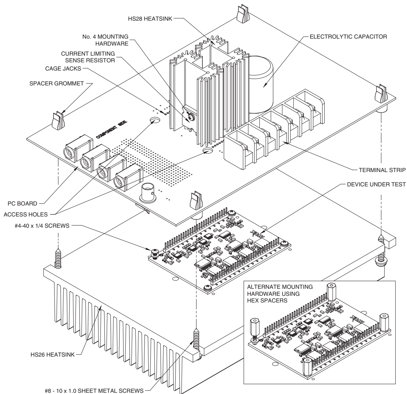
FIGURE 3: Assembly
