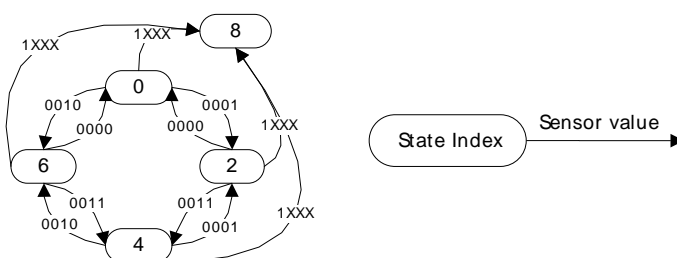
Figure 21.14. FSM example 2
