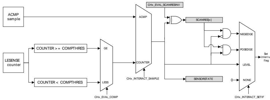
Figure 21.5. Scan result and interrupt generation
