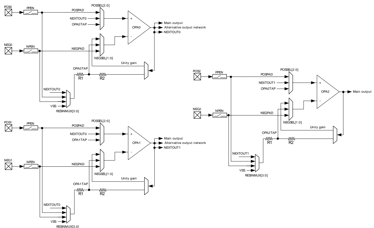
Figure 26.2. OPAMP Overview
