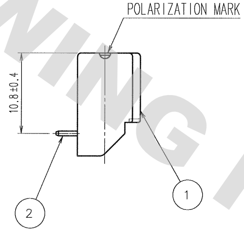
1 FOR DF1E-2P-2.5DS(01)
