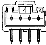
1 FOR DF1E-4P-2.5DS(01)
