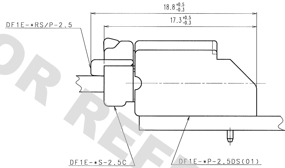
APPLICATION DIAGRAM(4:1)
