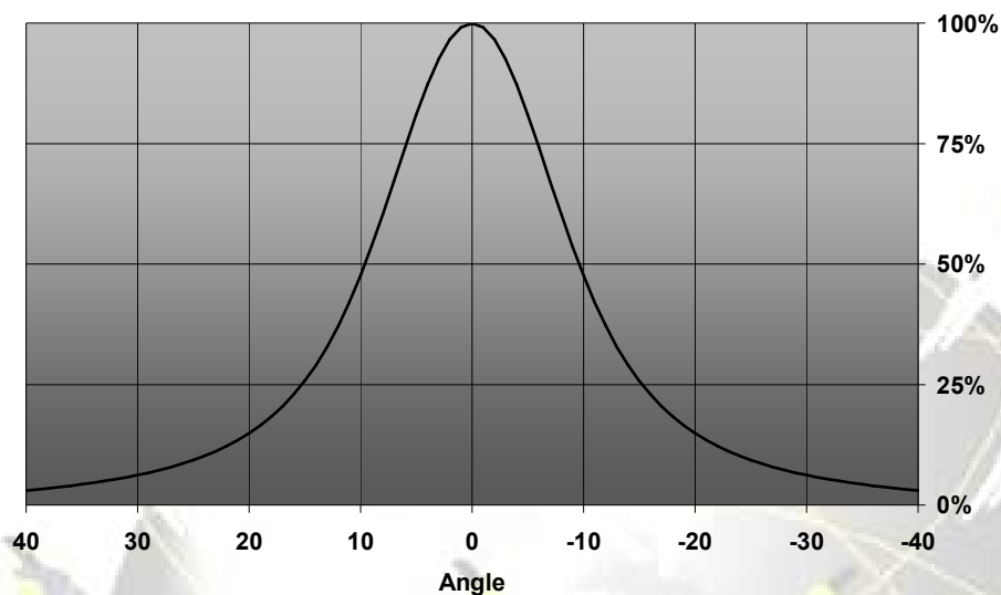
Relative Intensity of LISA-O1-SS
