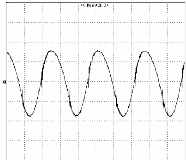
Figure 11: Input Terminal Ripple Current, i_c , at full rated output current and nominal input voltage with 12\mu H source impedance and 33\mu F electrolytic capacitor (200 mA/div, 1\mu s /div)
