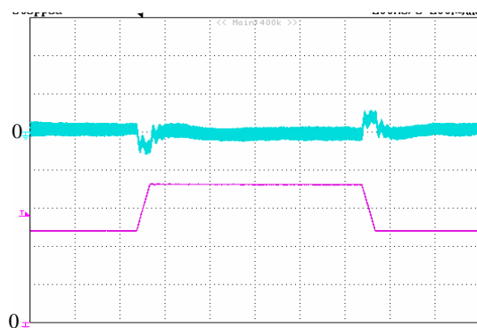
Figure 8: Output voltage response to step-change in load current (75%-50%-75% of I_o , max; di/dt = 0.1A/\mu s ). Load cap: 10 \mu F tantalum capacitor and 1 \mu F ceramic capacitor. Top Trace: V_{out} (100mV/div, 200us/div), Bottom Trace: I_{out} (5A/div). Scope measurement should be made using a BNC cable (length shorter than 20 inches). Position the load between 51 mm to 76 mm (2 inches to 3 inches) from the module
