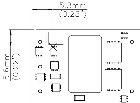
Figure 20: Temperature measurement location
