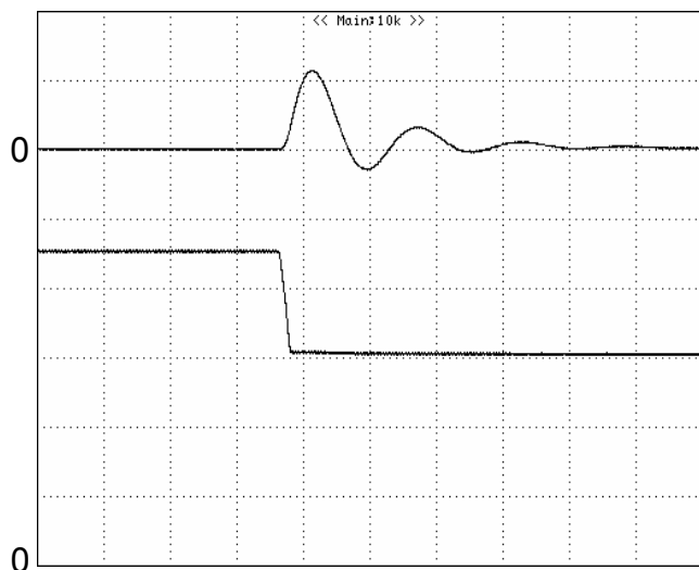
Figure 8: Output voltage response to step-change in load current (75%-50% of I_{O, max} ; di/dt = 0.1A/\mu s ). Load cap: 10\mu F tantalum capacitor and 1\mu F ceramic capacitor. Top Trace: V_{out} (200mV/div, 50us/div), Bottom Trace: I_{out} (0.5A/div). Scope measurement should be made using a BNC cable (length shorter than 20 inches). Position the load between 51 mm to 76 mm (2 inches to 3 inches) from the module
