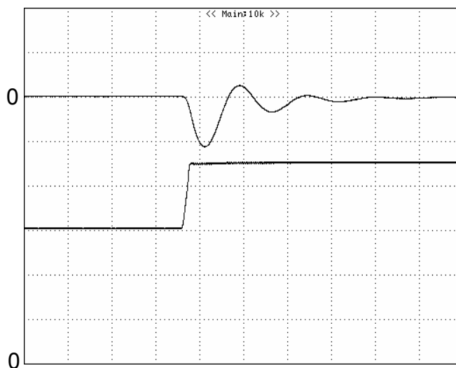
Figure 9: Output voltage response to step-change in load current (50%-75% of I_{O, max} ; di/dt = 0.1A/\mu s ). Load cap: 10\mu F tantalum capacitor and 1\mu F ceramic capacitor. Top Trace: V_{out} (200mV/div, 50us/div), Bottom Trace: I_{out} (0.5A/div). Scope measurement should be made using a BNC cable (length shorter than 20 inches). Position the load between 51 mm to 76 mm (2 inches to 3 inches) from the module
