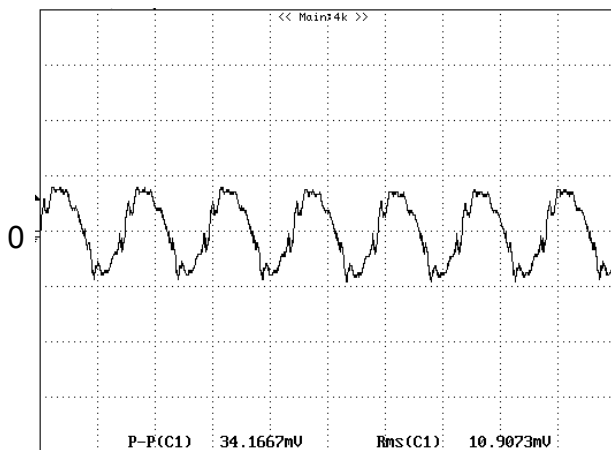
Figure 14: Output voltage ripple at nominal input voltage and rated load current ( I_o=5A ) (20 mV/div, 2μs/div) Load capacitance: 1μF ceramic capacitor and 10μF tantalum capacitor. Bandwidth: 20 MHz. Scope measurements should be made using a BNC cable (length shorter than 20 inches). Position the load between 51 mm to 76 mm (2 inches to 3 inches) from the module
