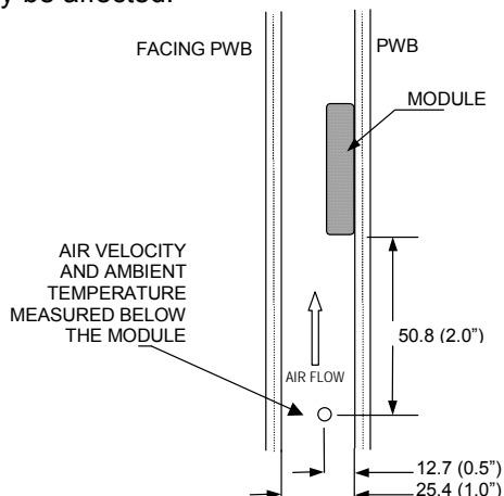
Figure 27: Wind tunnel test setup
