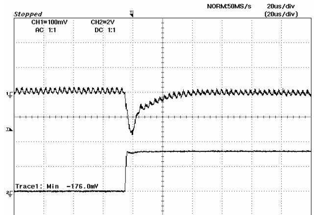
Figure 20: Typical transient response to step load change at 2.5A/\mu S from 50% to 100% of I_o , max at 5V_{in} , 3.3V_{out} ( C_{out} = 1\mu F ceramic, 10\mu F tantalum)
