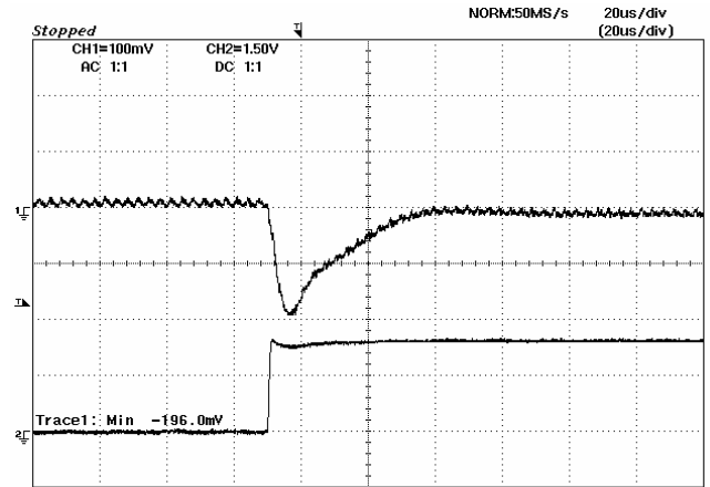
Figure 24: Typical transient response to step load change at 2.5A/\mu s from 50% to 100% of I_o , max at 3.3Vin, 2.5Vout (Cout = 1uF ceramic, 10uF tantalum)
