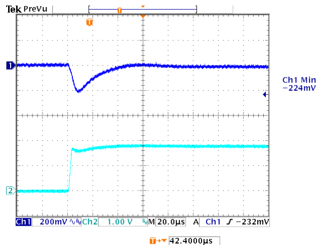
Figure 26: Typical Transient Response to Step Load Change at 2.5A/μs from 50% to 100% of I_o , max at 3.3Vin, 1.8Vout (Cout = 1μF ceramic, 10μF Tantalum)
