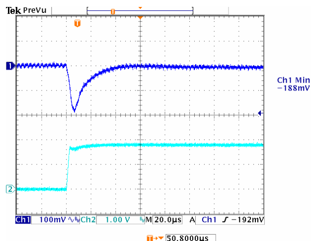
Figure 22: Typical Transient Response to Step Load Change at 2.5A/μs from 50% to 100% of I_o , max at 5Vin, 1.8Vout (Cout = 1μF ceramic, 10μF Tantalum)
