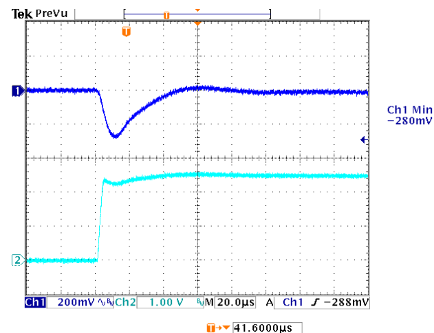
Figure 24: Typical Transient Response to Step Load Change at 2.5A/μs from 50% to 100% of I_o , max at 3.3Vin, 2.5Vout (Cout = 1μF ceramic, 10μF Tantalum)
