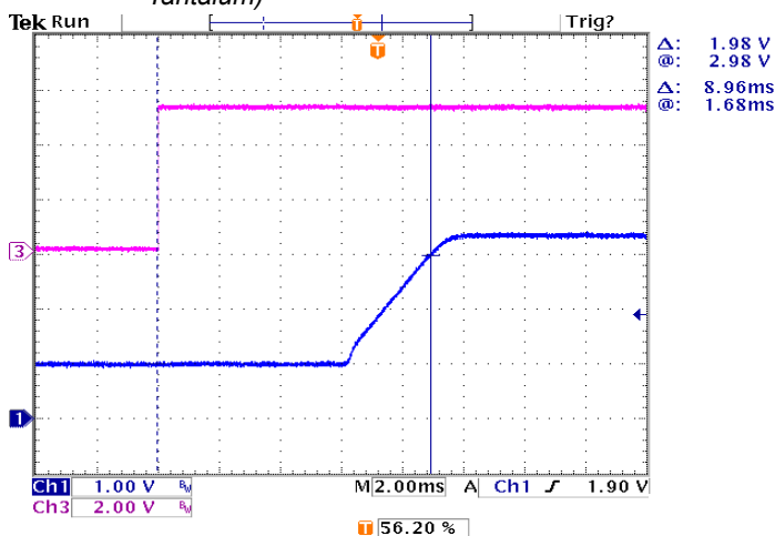
Figure 28: Turn on with Prebias 5Vin, 3.3V/0A out, Vbias = 1.0Vdc
