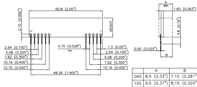
BACK VIEW
