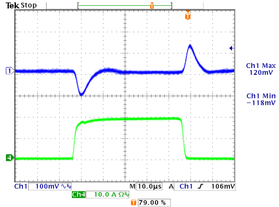
Figure 22: Typical transient response, 2.5V output CH1:Vo, Ch4:I0, 10A/div
