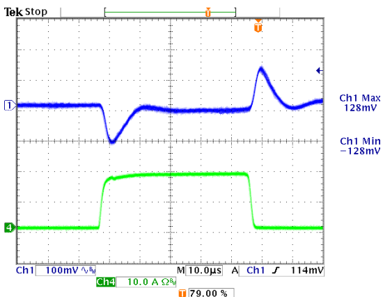
Figure 23: Typical transient response, 3.3V output CH1:Vo, Ch4:I0, 10A/div
