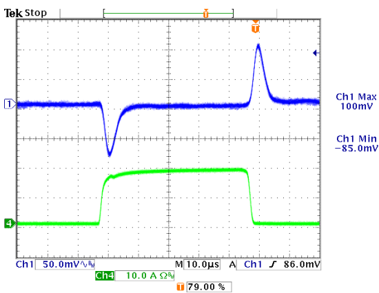
Figure 21: Typical transient response, 1.8V output CH1:Vo, Ch4:I0, 10A/div
