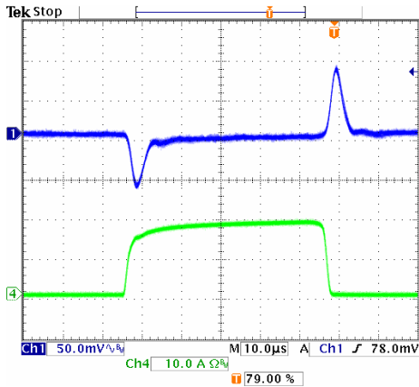
Figure 19: Typical transient response, 1.2V output CH1:Vo, Ch4:I0, 10A/div
