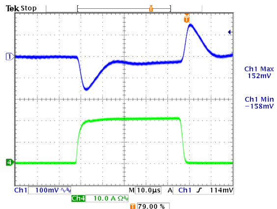
Figure 24: Typical transient response, 5.0V output CH1:Vo, Ch4:I0, 10A/div
