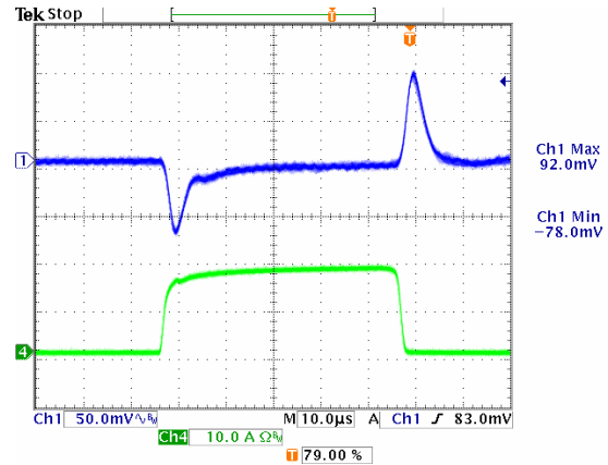
Figure 20: Typical transient response, 1.5V output CH1:Vo, Ch4:I0, 10A/div
