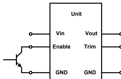
Figure 25: Enable Input drive circuit
