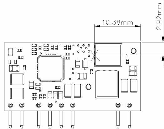
Figure 31: Temperature measurement location* The allowed maximum hot spot temperature is defined at 125 °C
