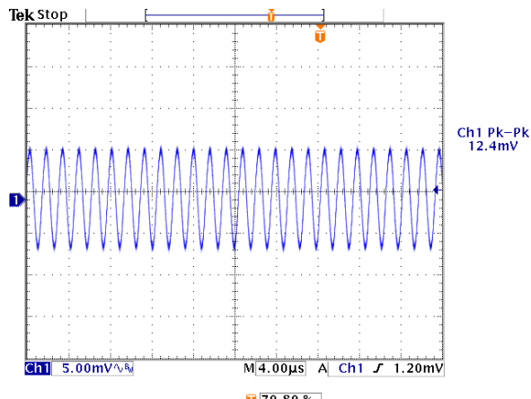
Figure 7: Output ripple & noise at 12Vin, 5.0V/20A out
