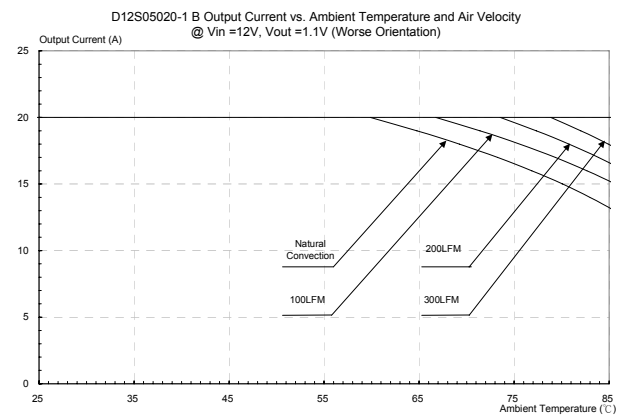
Figure 38: Output current vs. ambient temperature and air velocity @Vin=12V, Vout=1.1V (Worst Orientation)
