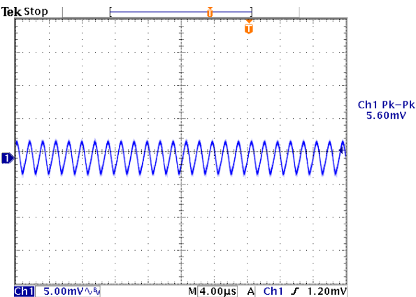
Figure 11: Output ripple & noise at 12Vin, 1.2V/20A out
