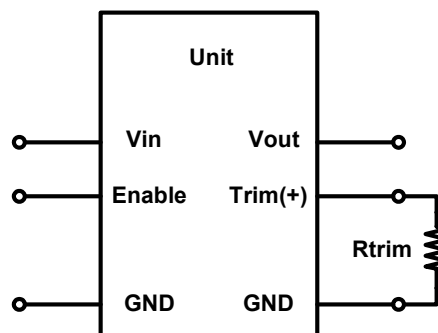
Figure 27: Trimming Output Voltage
