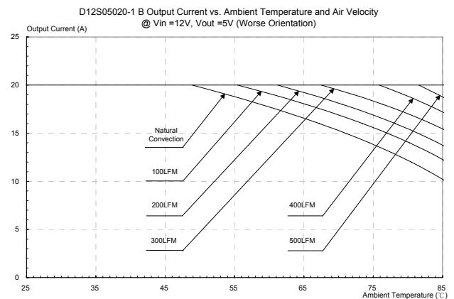
Figure 32: Output current vs. ambient temperature and air velocity @ Vin=12V, Vout=5.0V (Worst Orientation)
