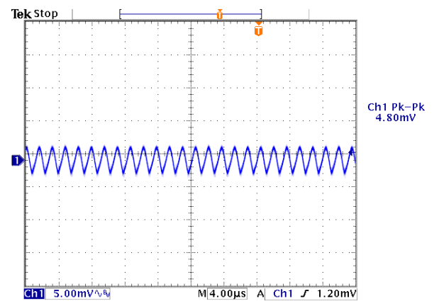
Figure 12: Output ripple & noise at 12Vin, 0.9V/20A out
