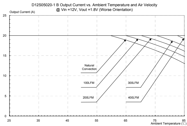
Figure 35: Output current vs. ambient temperature and air velocity @Vin=12V, Vout=1.8V (Worst Orientation)
