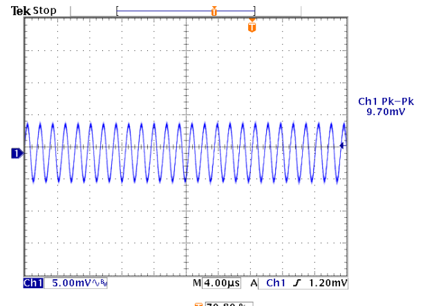
Figure 8: Output ripple & noise at 12Vin, 3.3V/20A out
