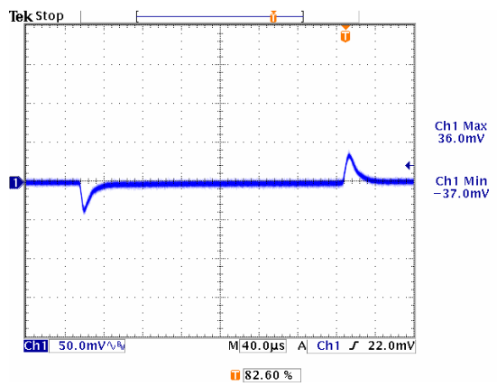
Figure 22: Transient response, 1.5V /20A, Ch1: Vo
