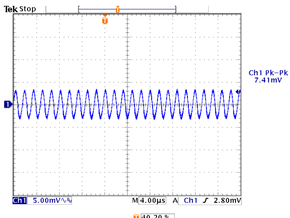
Figure 9: Output ripple & noise at 12Vin, 2.5V/20A out
