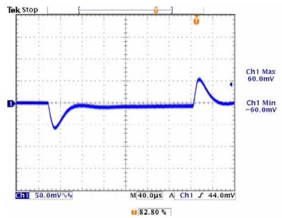
Figure 20: Transient response, 3.3V /20A, Ch1: Vo
