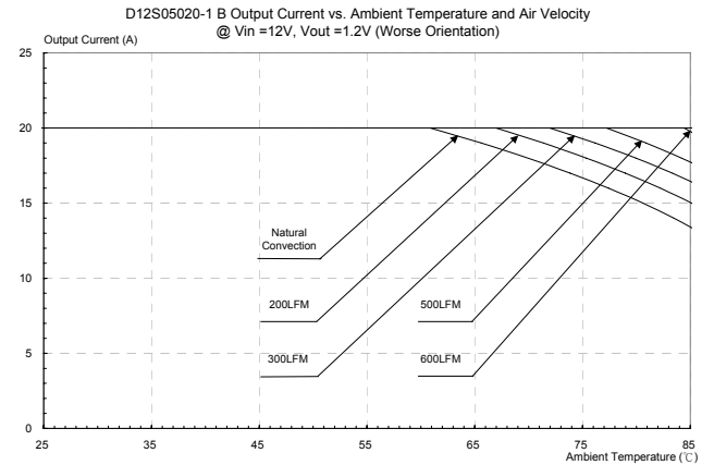
Figure 37: Output current vs. ambient temperature and air velocity@ Vin=12V, Vout=1.2V (Worst Orientation)
