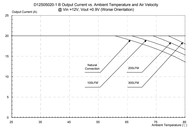
Figure 39: Output current vs. ambient temperature and air velocity @Vin=12V, Vout=0.9 V (Worst Orientation)
