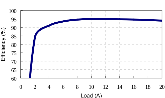
Figure 1: Converter efficiency vs. output current (5.0V output voltage, 12V input)
