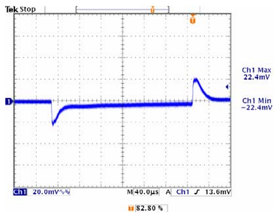
Figure 23: Transient response, 1.2V /20A, Ch1: Vo
