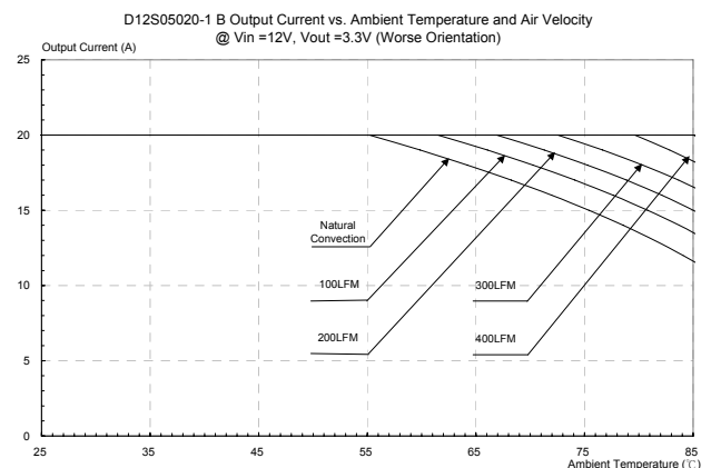
Figure 33: Output current vs. ambient temperature and air velocity @ Vin=12V, Vout=3.3V (Worst Orientation)
