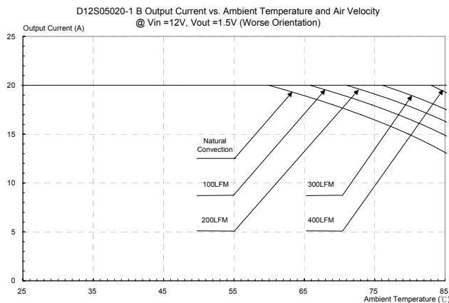
Figure 36: Output current vs. ambient temperature and air velocity@ Vin=12V, Vout=1.5V (Worst Orientation)
