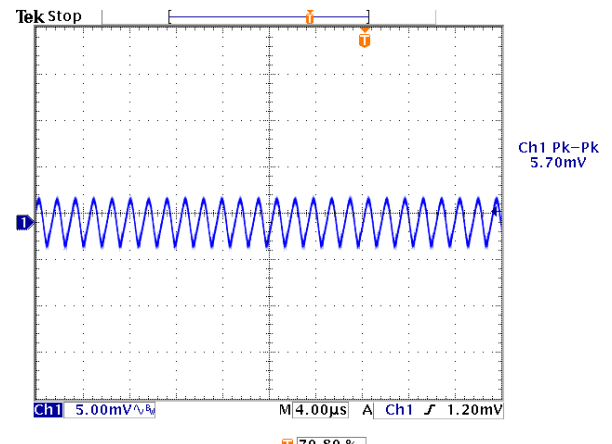
Figure 10: Output ripple & noise at 12Vin, 1.5V/20A out
