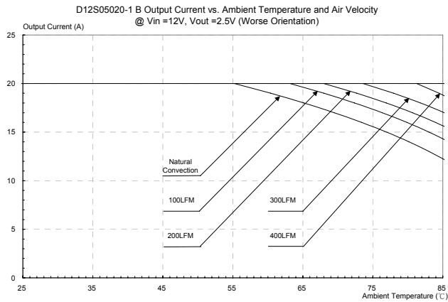
Figure 34: Output current vs. ambient temperature and air velocity@ Vin=12V, Vout=2.5V (Worst Orientation)
