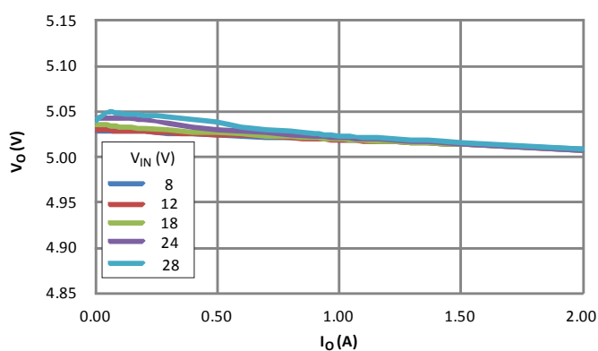
Load Regulation versus Output Current
