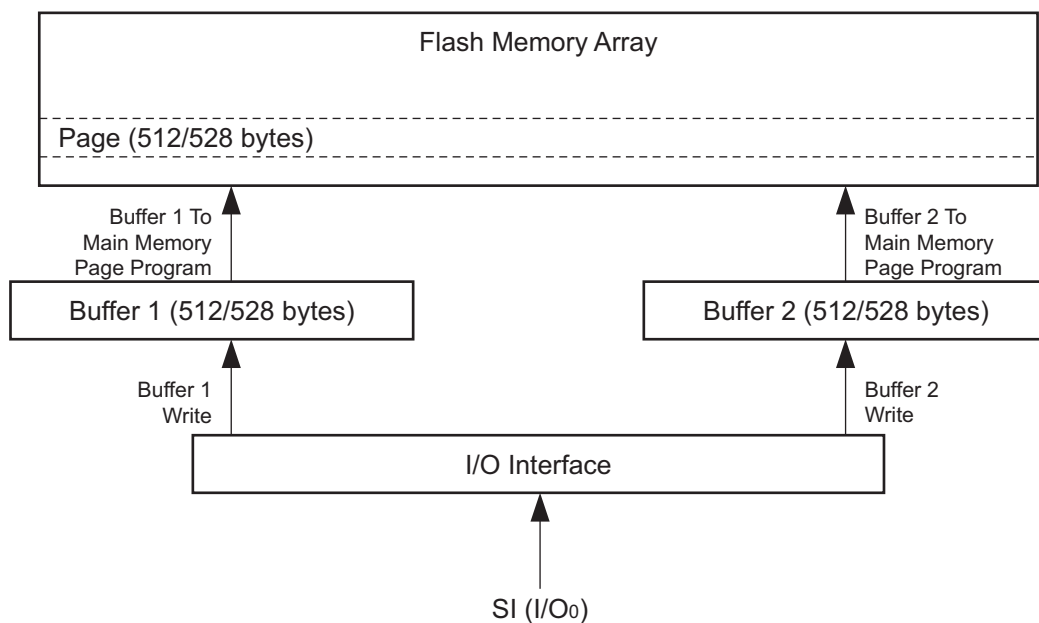
Figure 23-1. Block Diagram
