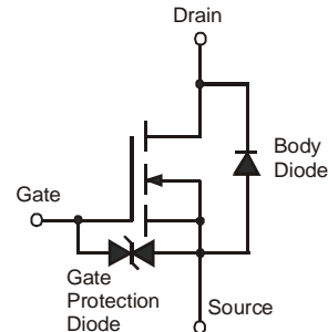
Equivalent Circuit
