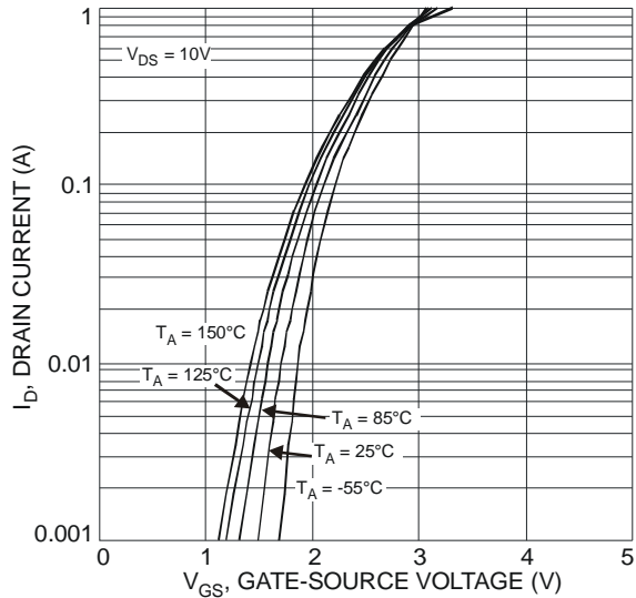
Fig. 9 Typical Transfer Characteristic
