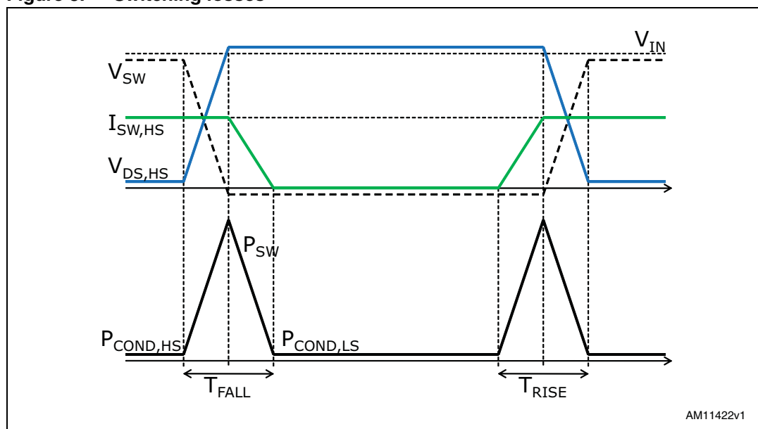
Figure 8. Switching losses
