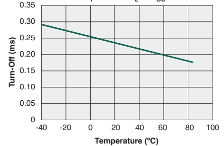
Typical Turn-Off vs. Temperature ( I_F=10\text{mA} , I_L=1A_{DC} )
