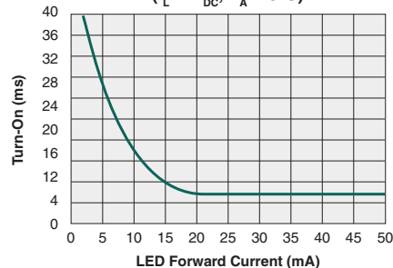
Typical Turn-On vs. LED Forward Current ( I_L=1A_{DC} , T_A=25^\circ\text{C} )
